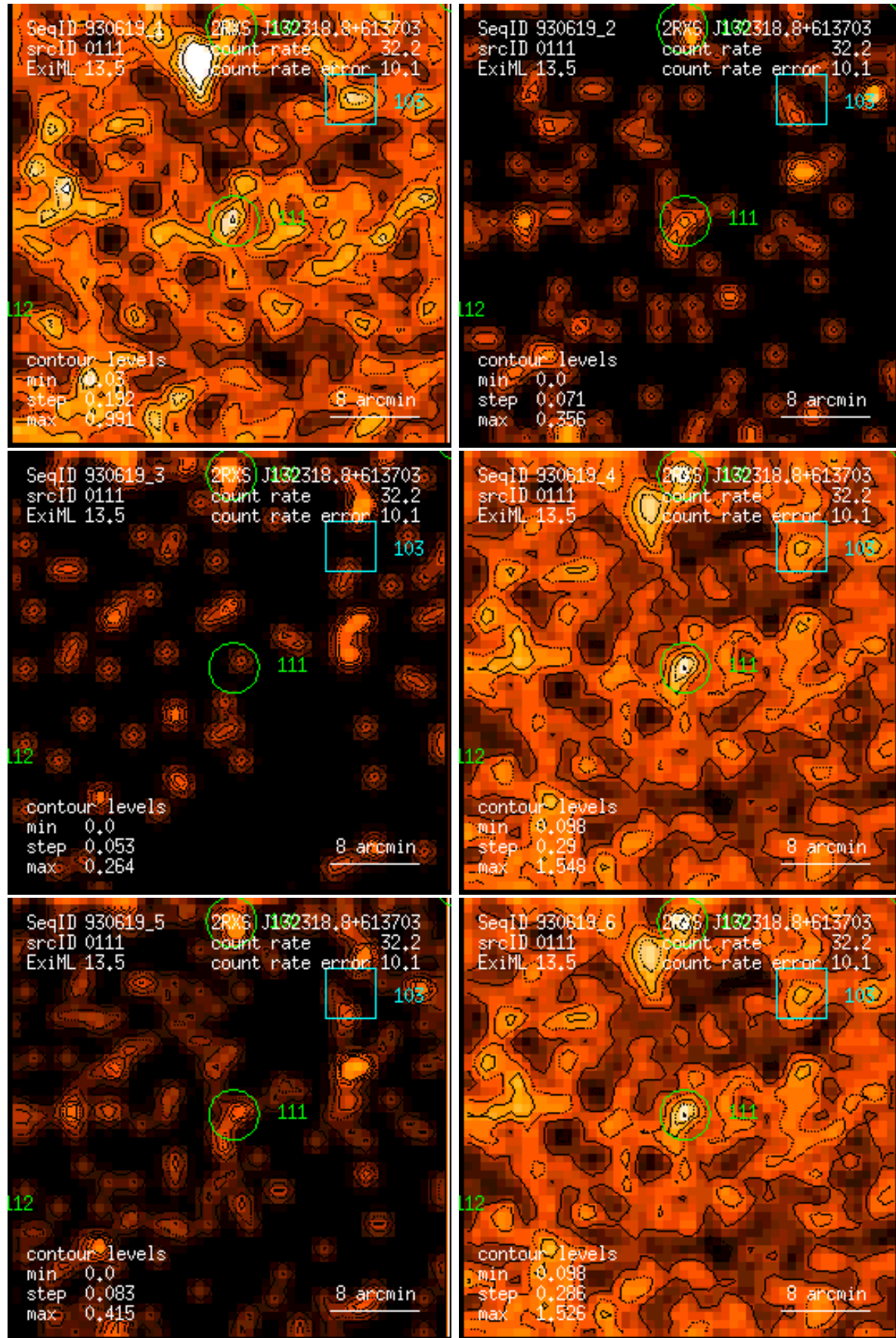
Figure 111: RASS 930619: detection 0111: band rate images, Gaussian filter: (1) PSPC channels 11 – 41, (2) 52 – 90, (3) 91 – 201, (4) 11 – 235, (5) 52 – 201, (6) 11 – 201. Broad band rates in counts/ks. Band rate contour levels in counts/ks/arcmin 2 .
