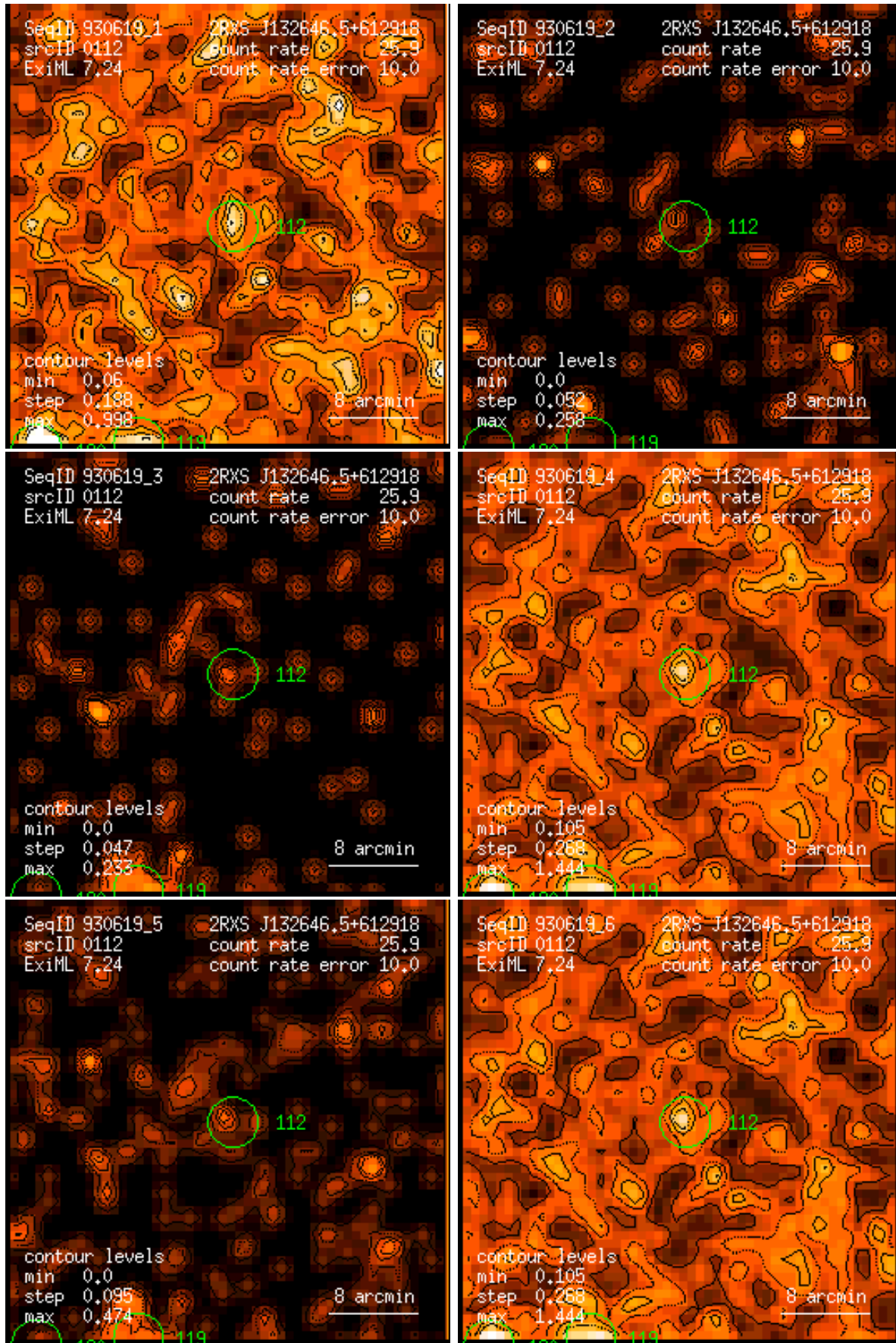
Figure 112: RASS 930619: detection 0112: band rate images, Gaussian filter: (1) PSPC channels 11 – 41, (2) 52 – 90, (3) 91 – 201, (4) 11 – 235, (5) 52 – 201, (6) 11 – 201. Broad band rates in counts/ks. Band rate contour levels in counts/ks/arcmin 2 .
