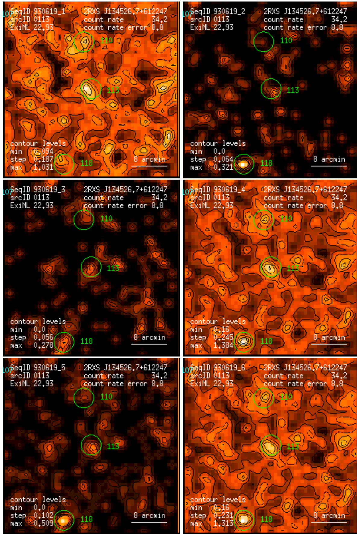
Figure 113: RASS 930619: detection 0113: band rate images, Gaussian filter: (1) PSPC channels 11 – 41, (2) 52 – 90, (3) 91 – 201, (4) 11 – 235, (5) 52 – 201, (6) 11 – 201. Broad band rates in counts/ks. Band rate contour levels in counts/ks/arcmin 2 .
