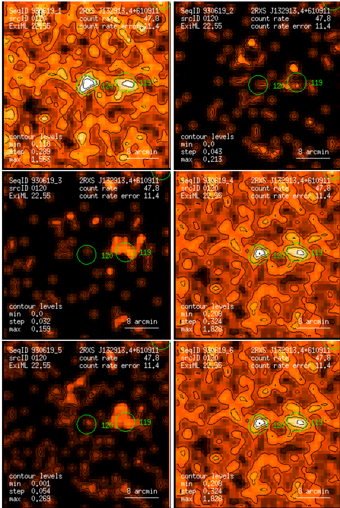
Figure 120: RASS 930619: detection 0120: band rate images, Gaussian filter: (1) PSPC channels 11 – 41, (2) 52 – 90, (3) 91 – 201, (4) 11 – 235, (5) 52 – 201, (6) 11 – 201. Broad band rates in counts/ks. Band rate contour levels in counts/ks/arcmin 2 .
