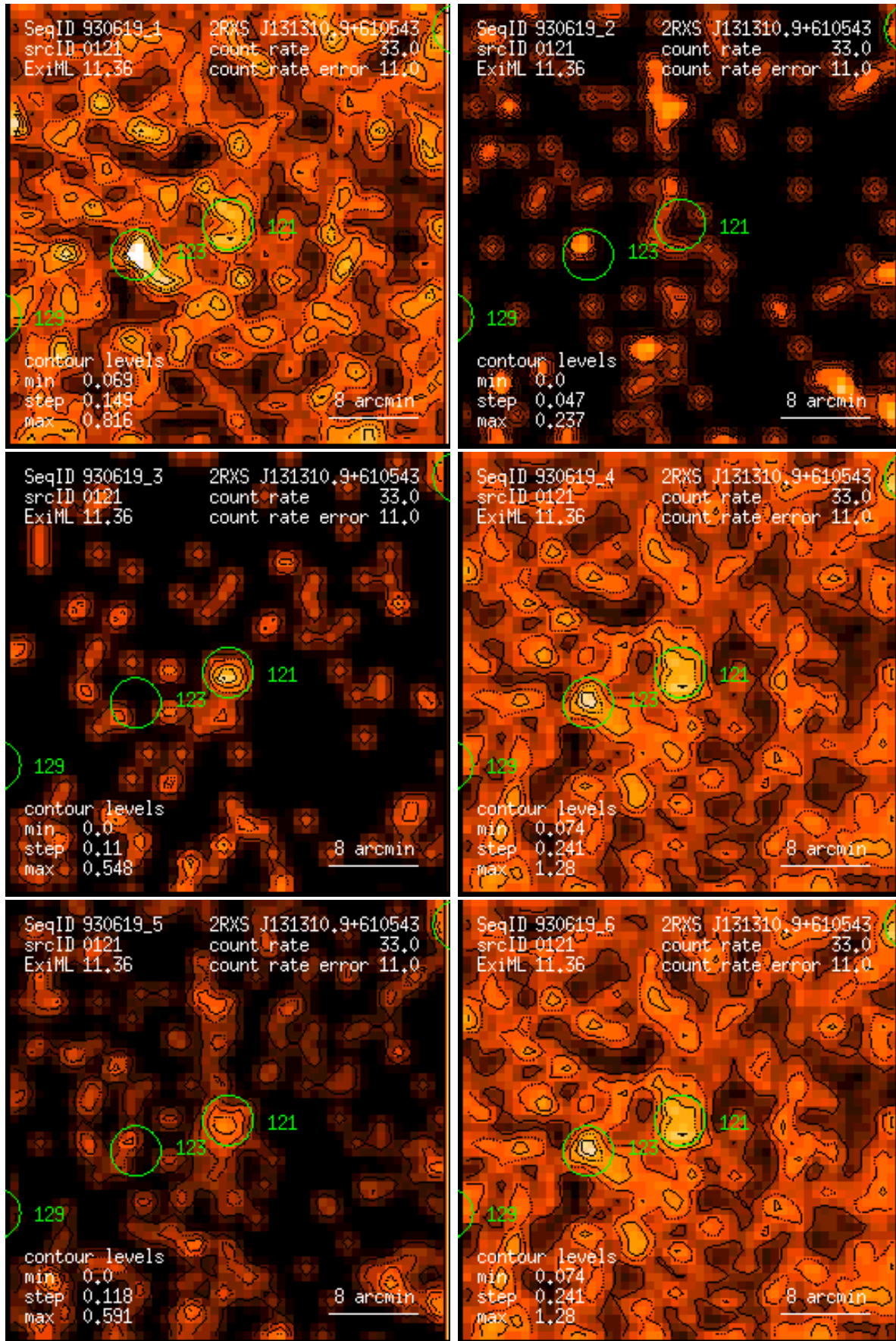
Figure 121: RASS 930619: detection 0121: band rate images, Gaussian filter: (1) PSPC channels 11 – 41, (2) 52 – 90, (3) 91 – 201, (4) 11 – 235, (5) 52 – 201, (6) 11 – 201. Broad band rates in counts/ks. Band rate contour levels in counts/ks/arcmin 2 .
