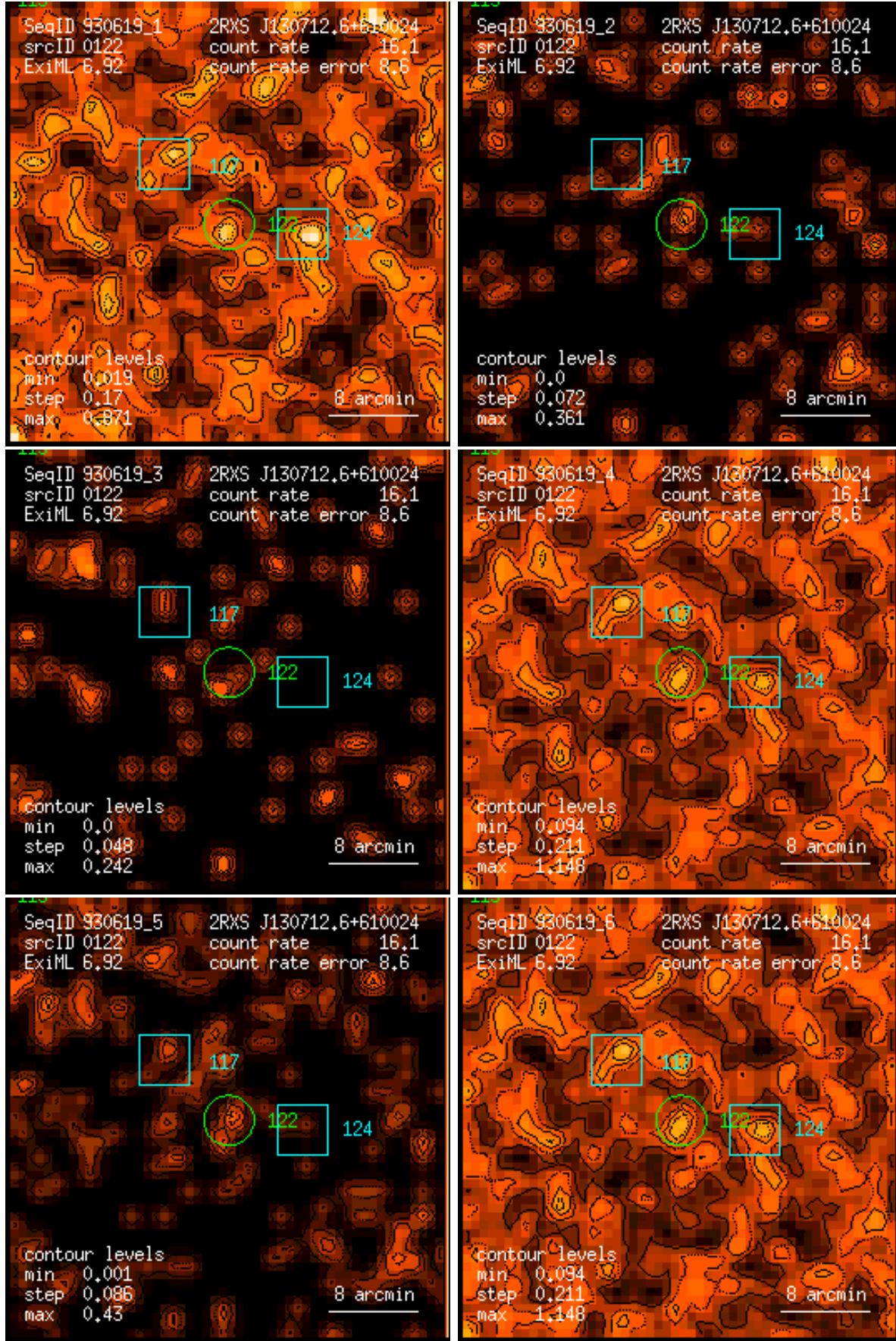
Figure 122: RASS 930619: detection 0122: band rate images, Gaussian filter: (1) PSPC channels 11 – 41, (2) 52 – 90, (3) 91 – 201, (4) 11 – 235, (5) 52 – 201, (6) 11 – 201. Broad band rates in counts/ks. Band rate contour levels in counts/ks/arcmin 2 .
