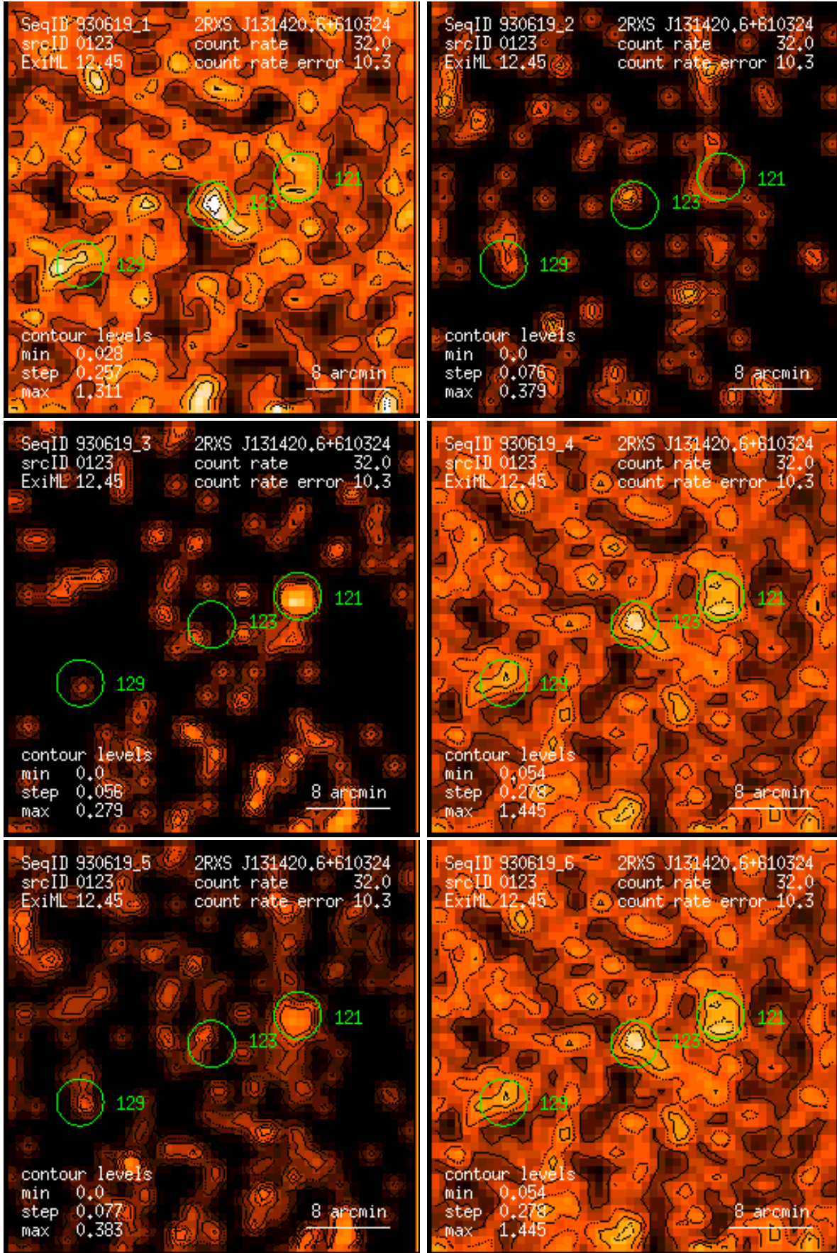
Figure 123: RASS 930619: detection 0123: band rate images, Gaussian filter: (1) PSPC channels 11 – 41, (2) 52 – 90, (3) 91 – 201, (4) 11 – 235, (5) 52 – 201, (6) 11 – 201. Broad band rates in counts/ks. Band rate contour levels in counts/ks/arcmin 2 .
