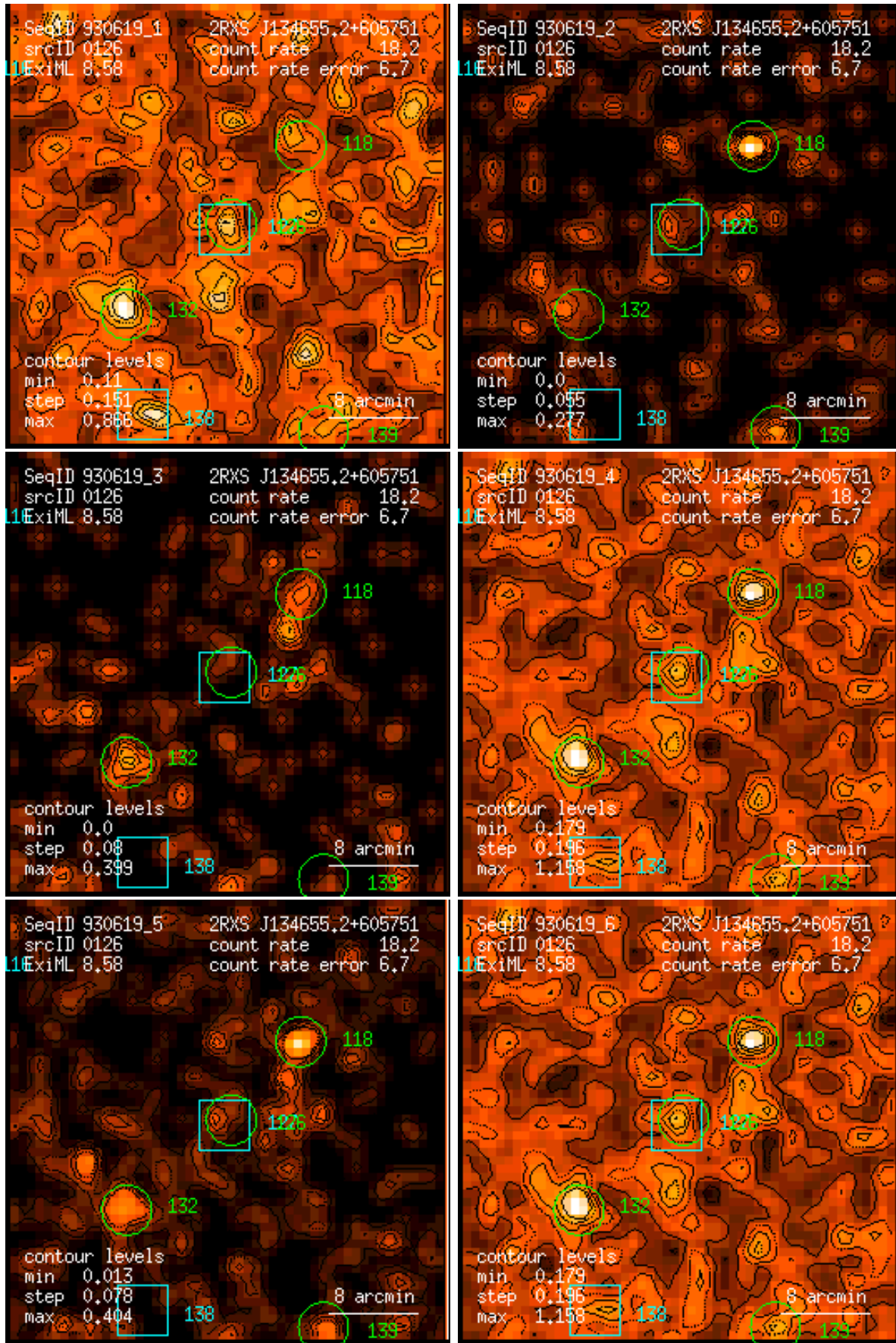
Figure 126: RASS 930619: detection 0126: band rate images, Gaussian filter: (1) PSPC channels 11 – 41, (2) 52 – 90, (3) 91 – 201, (4) 11 – 235, (5) 52 – 201, (6) 11 – 201. Broad band rates in counts/ks. Band rate contour levels in counts/ks/arcmin 2 .
