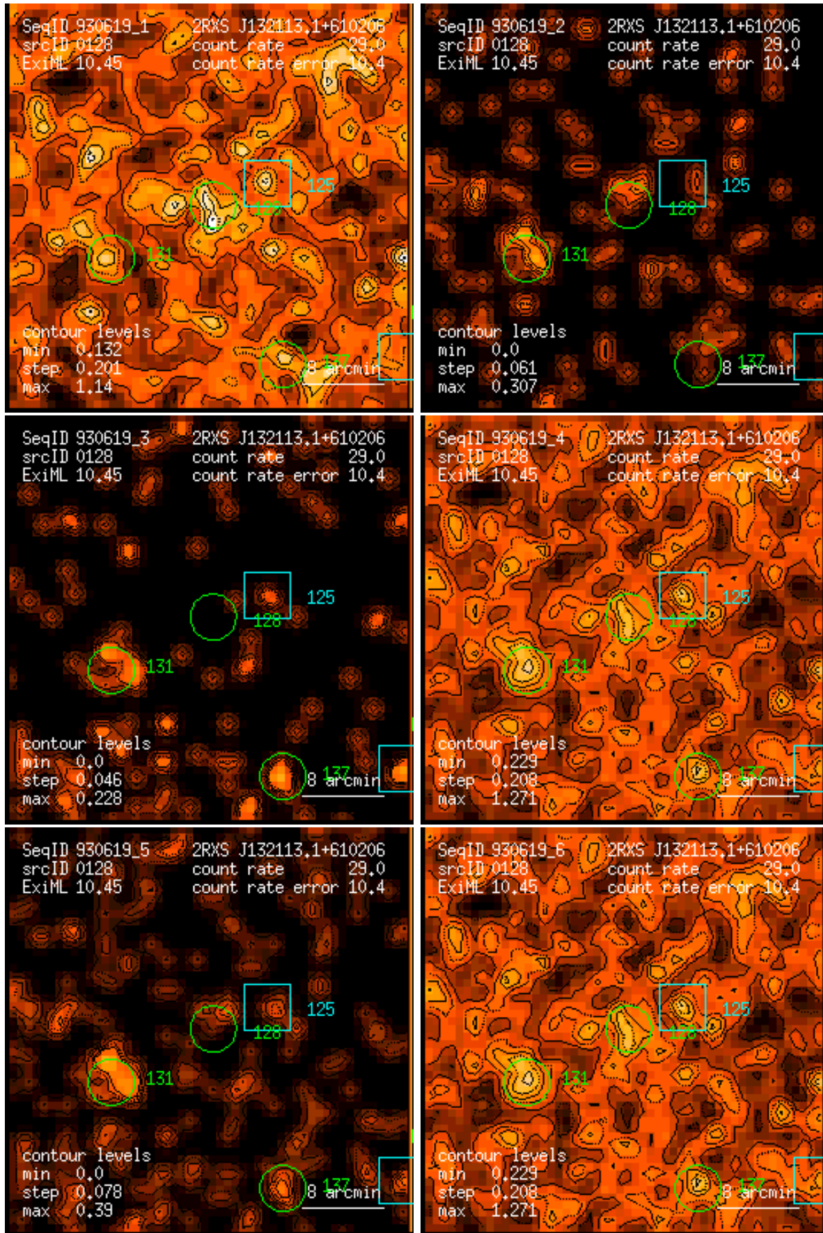
Figure 128: RASS 930619: detection 0128: band rate images, Gaussian filter: (1) PSPC channels 11 – 41, (2) 52 – 90, (3) 91 – 201, (4) 11 – 235, (5) 52 – 201, (6) 11 – 201. Broad band rates in counts/ks. Band rate contour levels in counts/ks/arcmin 2 .
