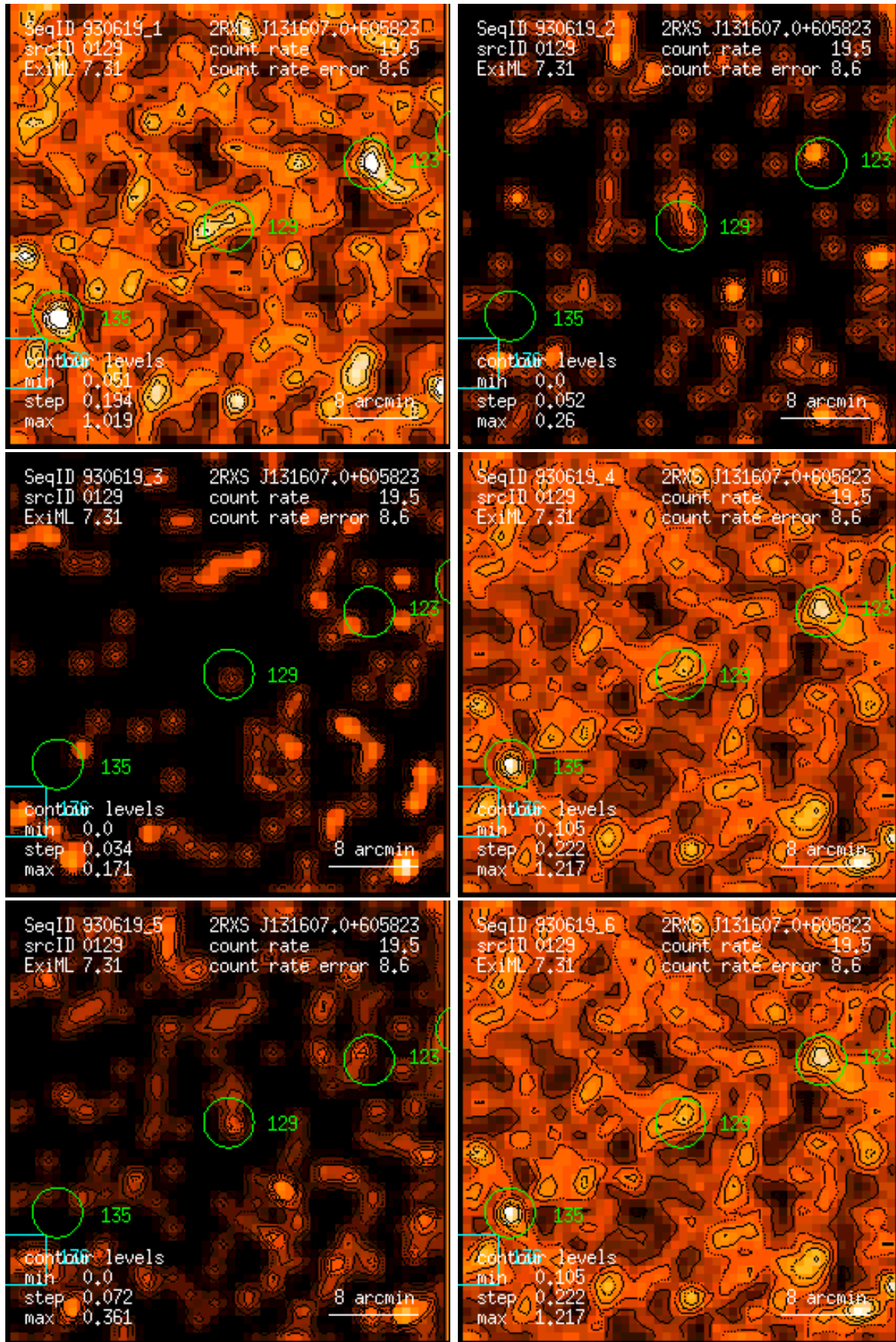
Figure 129: RASS 930619: detection 0129: band rate images, Gaussian filter: (1) PSPC channels 11 – 41, (2) 52 – 90, (3) 91 – 201, (4) 11 – 235, (5) 52 – 201, (6) 11 – 201. Broad band rates in counts/ks. Band rate contour levels in counts/ks/arcmin 2 .
