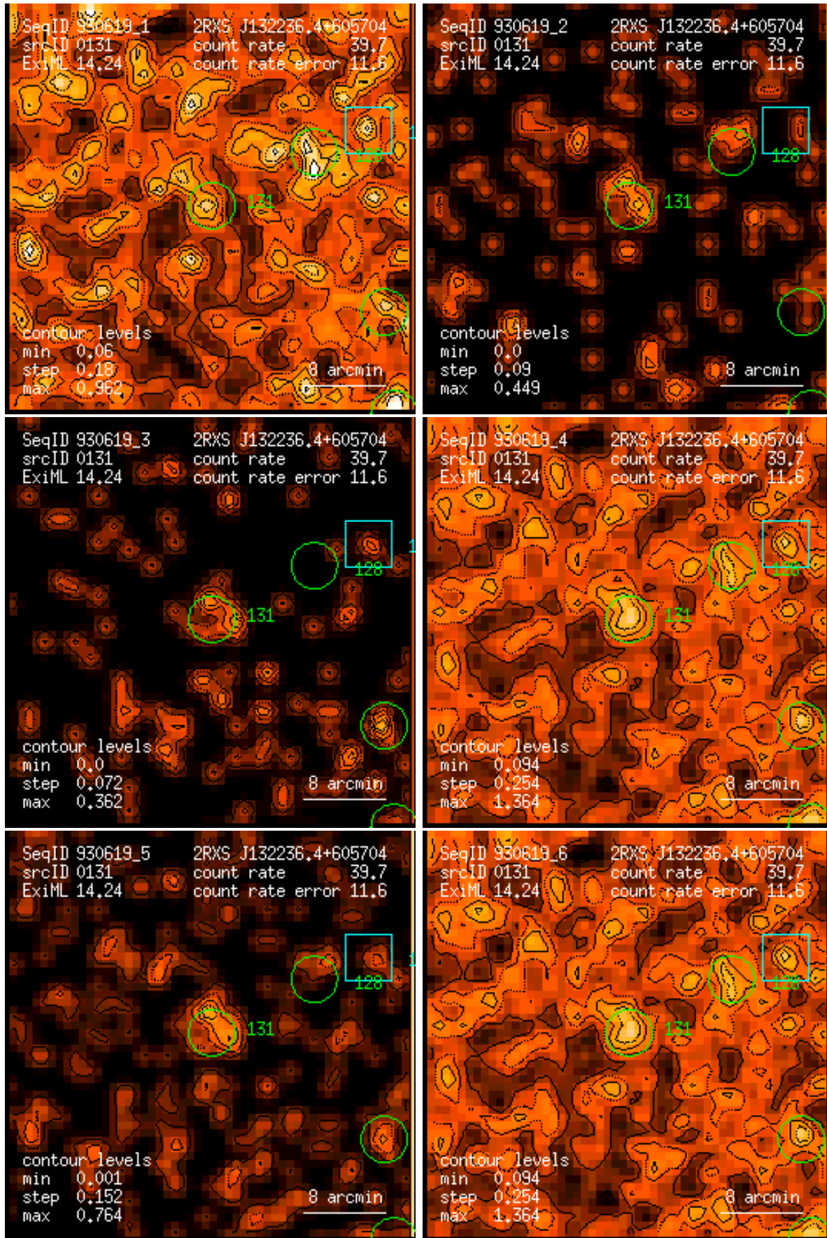
Figure 131: RASS 930619: detection 0131: band rate images, Gaussian filter: (1) PSPC channels 11 – 41, (2) 52 – 90, (3) 91 – 201, (4) 11 – 235, (5) 52 – 201, (6) 11 – 201. Broad band rates in counts/ks. Band rate contour levels in counts/ks/arcmin 2 .
