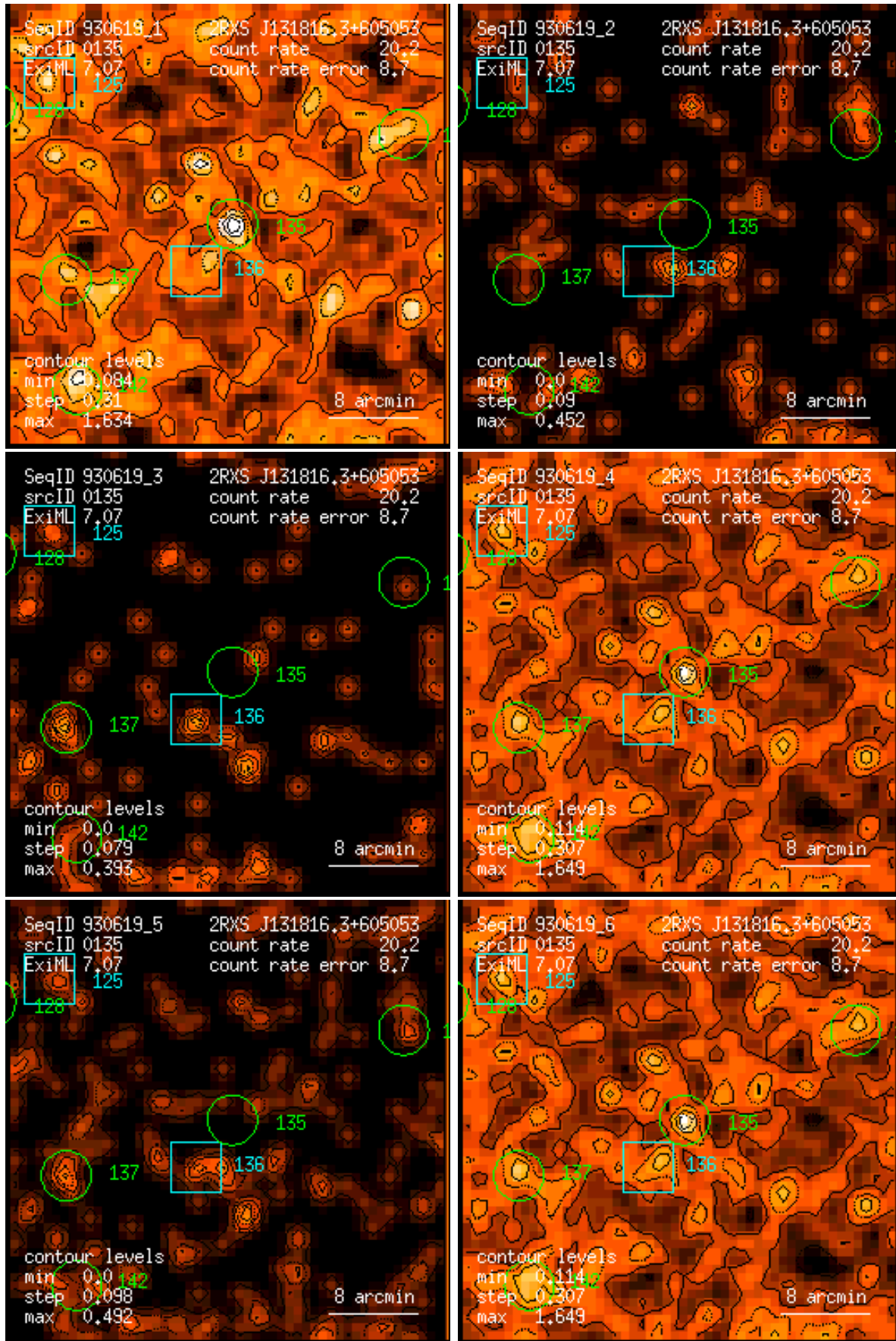
Figure 135: RASS 930619: detection 0135: band rate images, Gaussian filter: (1) PSPC channels 11 – 41, (2) 52 – 90, (3) 91 – 201, (4) 11 – 235, (5) 52 – 201, (6) 11 – 201. Broad band rates in counts/ks. Band rate contour levels in counts/ks/arcmin 2 .
