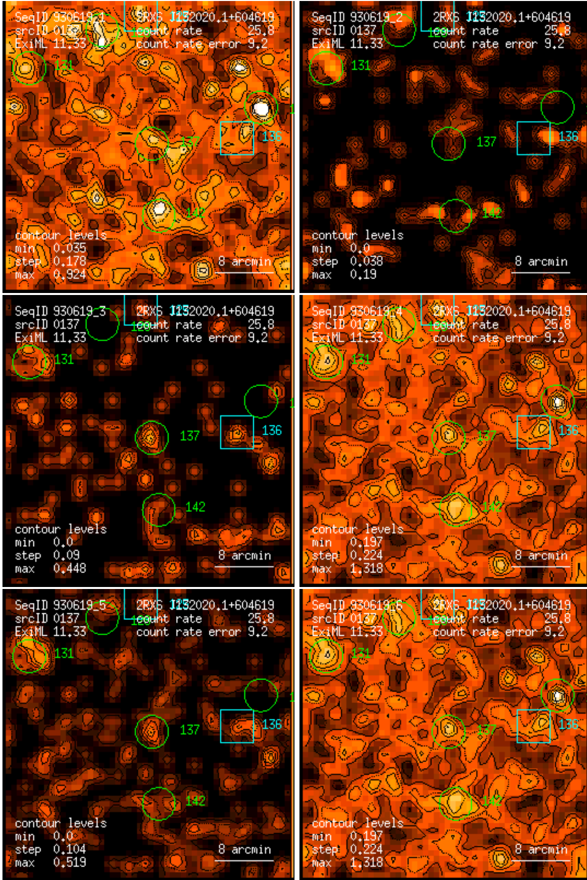
Figure 137: RASS 930619: detection 0137: band rate images, Gaussian filter: (1) PSPC channels 11 – 41, (2) 52 – 90, (3) 91 – 201, (4) 11 – 235, (5) 52 – 201, (6) 11 – 201. Broad band rates in counts/ks. Band rate contour levels in counts/ks/arcmin 2 .
