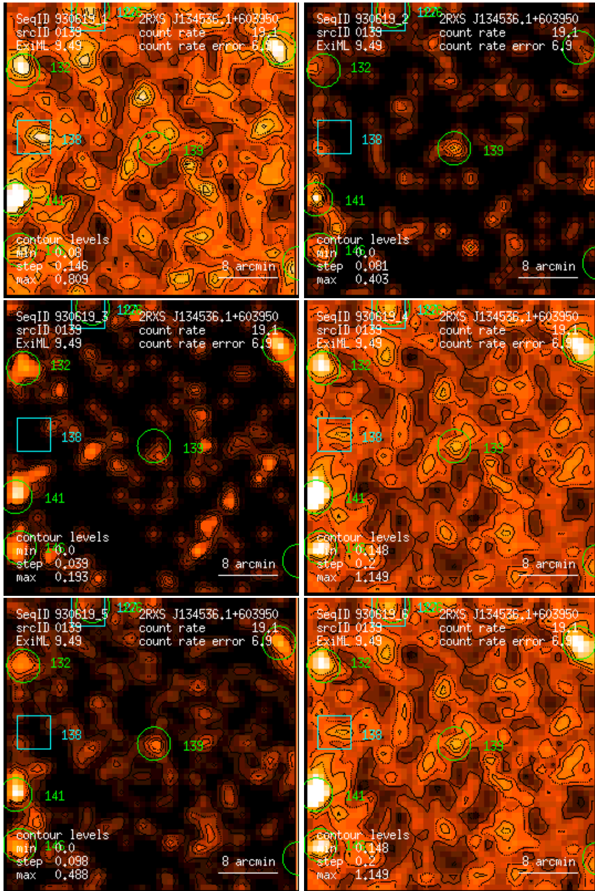
Figure 139: RASS 930619: detection 0139: band rate images, Gaussian filter: (1) PSPC channels 11 – 41, (2) 52 – 90, (3) 91 – 201, (4) 11 – 235, (5) 52 – 201, (6) 11 – 201. Broad band rates in counts/ks. Band rate contour levels in counts/ks/arcmin 2 .
