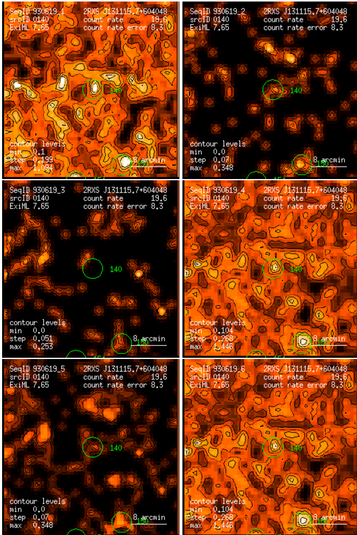
Figure 140: RASS 930619: detection 0140: band rate images, Gaussian filter: (1) PSPC channels 11 – 41, (2) 52 – 90, (3) 91 – 201, (4) 11 – 235, (5) 52 – 201, (6) 11 – 201. Broad band rates in counts/ks. Band rate contour levels in counts/ks/arcmin 2 .
