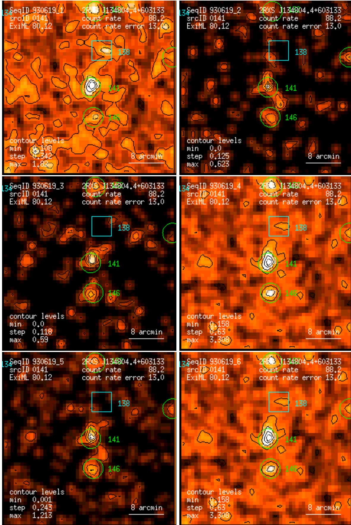
Figure 141: RASS 930619: detection 0141: band rate images, Gaussian filter: (1) PSPC channels 11 – 41, (2) 52 – 90, (3) 91 – 201, (4) 11 – 235, (5) 52 – 201, (6) 11 – 201. Broad band rates in counts/ks. Band rate contour levels in counts/ks/arcmin 2 .
