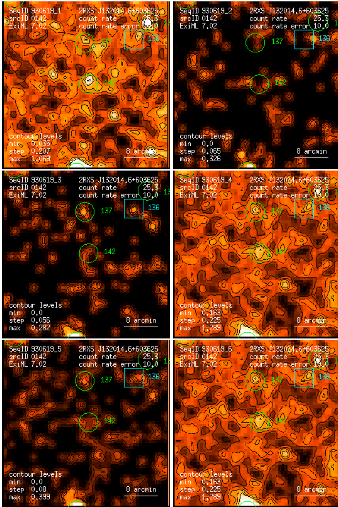
Figure 142: RASS 930619: detection 0142: band rate images, Gaussian filter: (1) PSPC channels 11 – 41, (2) 52 – 90, (3) 91 – 201, (4) 11 – 235, (5) 52 – 201, (6) 11 – 201. Broad band rates in counts/ks. Band rate contour levels in counts/ks/arcmin 2 .
