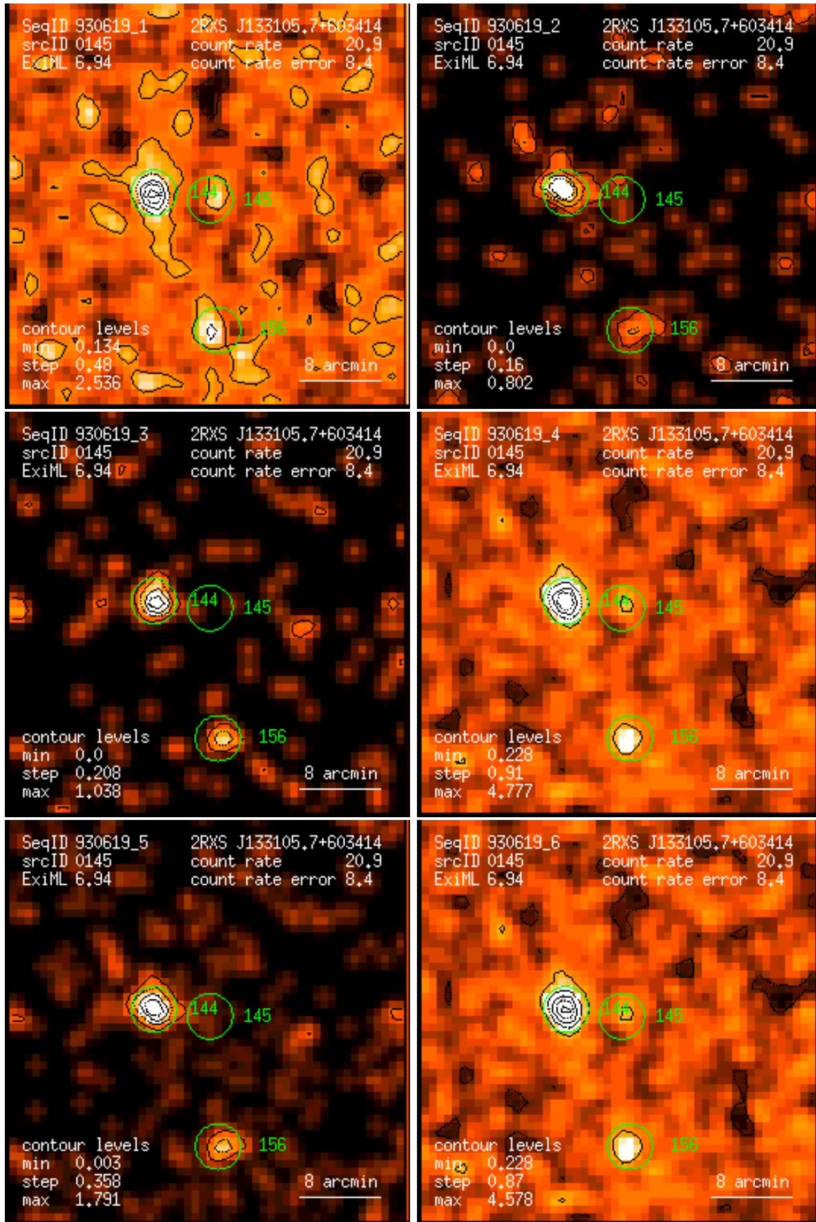
Figure 145: RASS 930619: detection 0145: band rate images, Gaussian filter: (1) PSPC channels 11 – 41, (2) 52 – 90, (3) 91 – 201, (4) 11 – 235, (5) 52 – 201, (6) 11 – 201. Broad band rates in counts/ks. Band rate contour levels in counts/ks/arcmin 2 .
