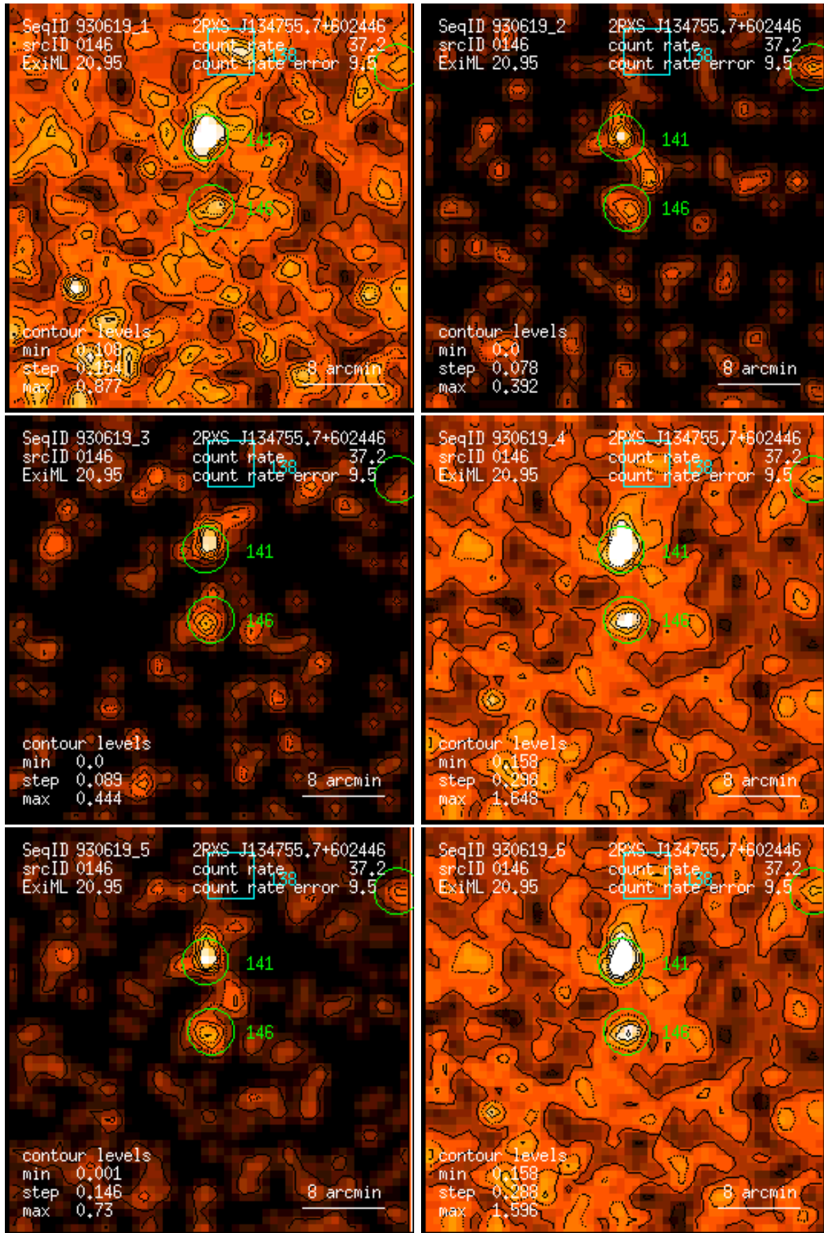
Figure 146: RASS 930619: detection 0146: band rate images, Gaussian filter: (1) PSPC channels 11 – 41, (2) 52 – 90, (3) 91 – 201, (4) 11 – 235, (5) 52 – 201, (6) 11 – 201. Broad band rates in counts/ks. Band rate contour levels in counts/ks/arcmin 2 .
