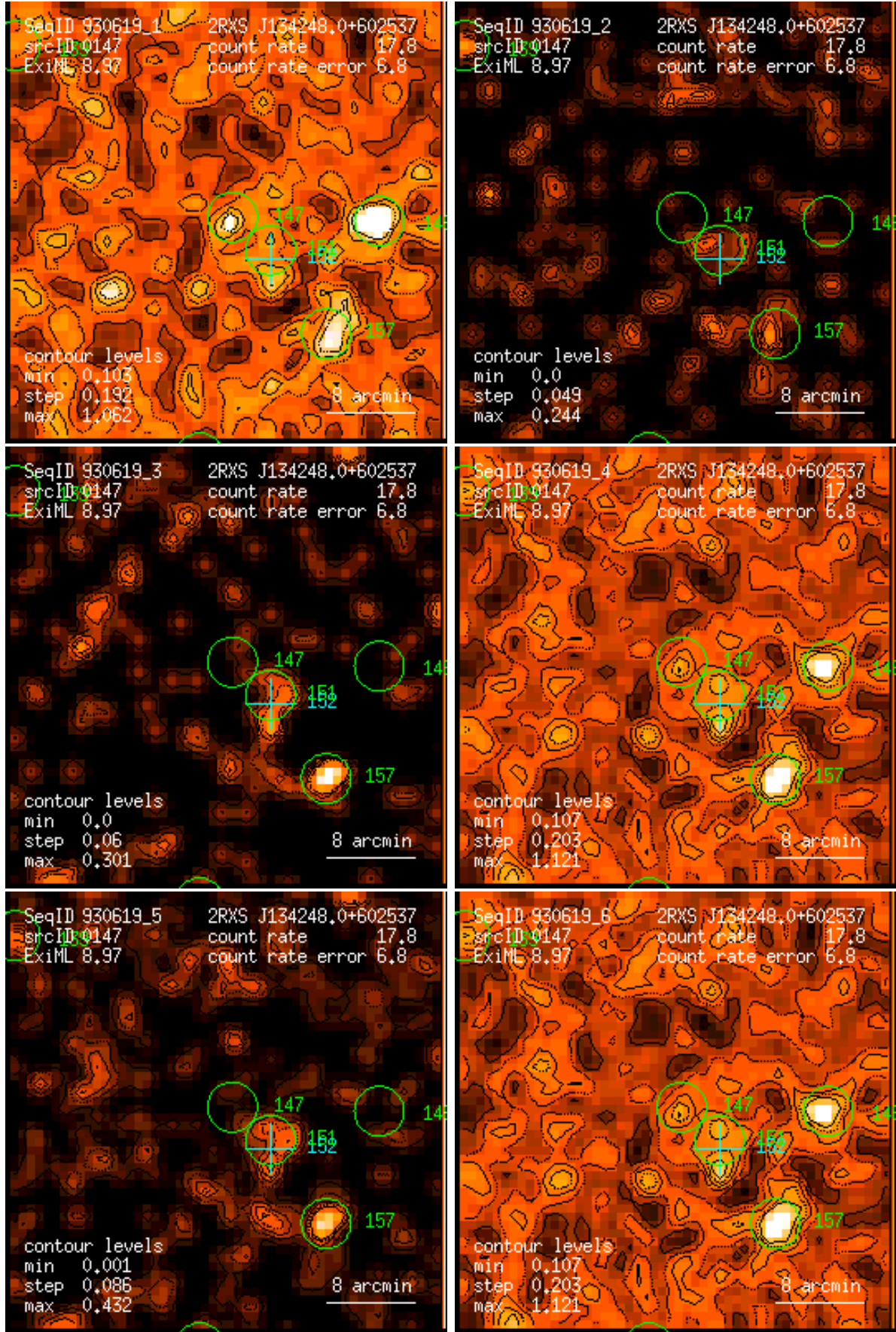
Figure 147: RASS 930619: detection 0147: band rate images, Gaussian filter: (1) PSPC channels 11 – 41, (2) 52 – 90, (3) 91 – 201, (4) 11 – 235, (5) 52 – 201, (6) 11 – 201. Broad band rates in counts/ks. Band rate contour levels in counts/ks/arcmin 2 .
