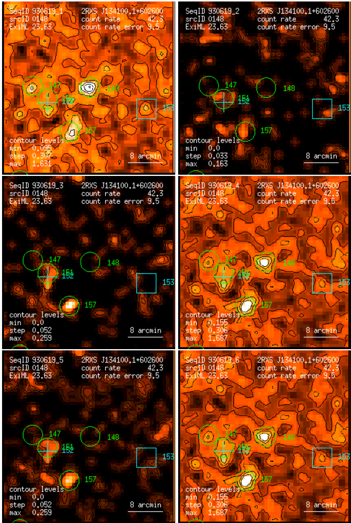
Figure 148: RASS 930619: detection 0148: band rate images, Gaussian filter: (1) PSPC channels 11 – 41, (2) 52 – 90, (3) 91 – 201, (4) 11 – 235, (5) 52 – 201, (6) 11 – 201. Broad band rates in counts/ks. Band rate contour levels in counts/ks/arcmin 2 .
