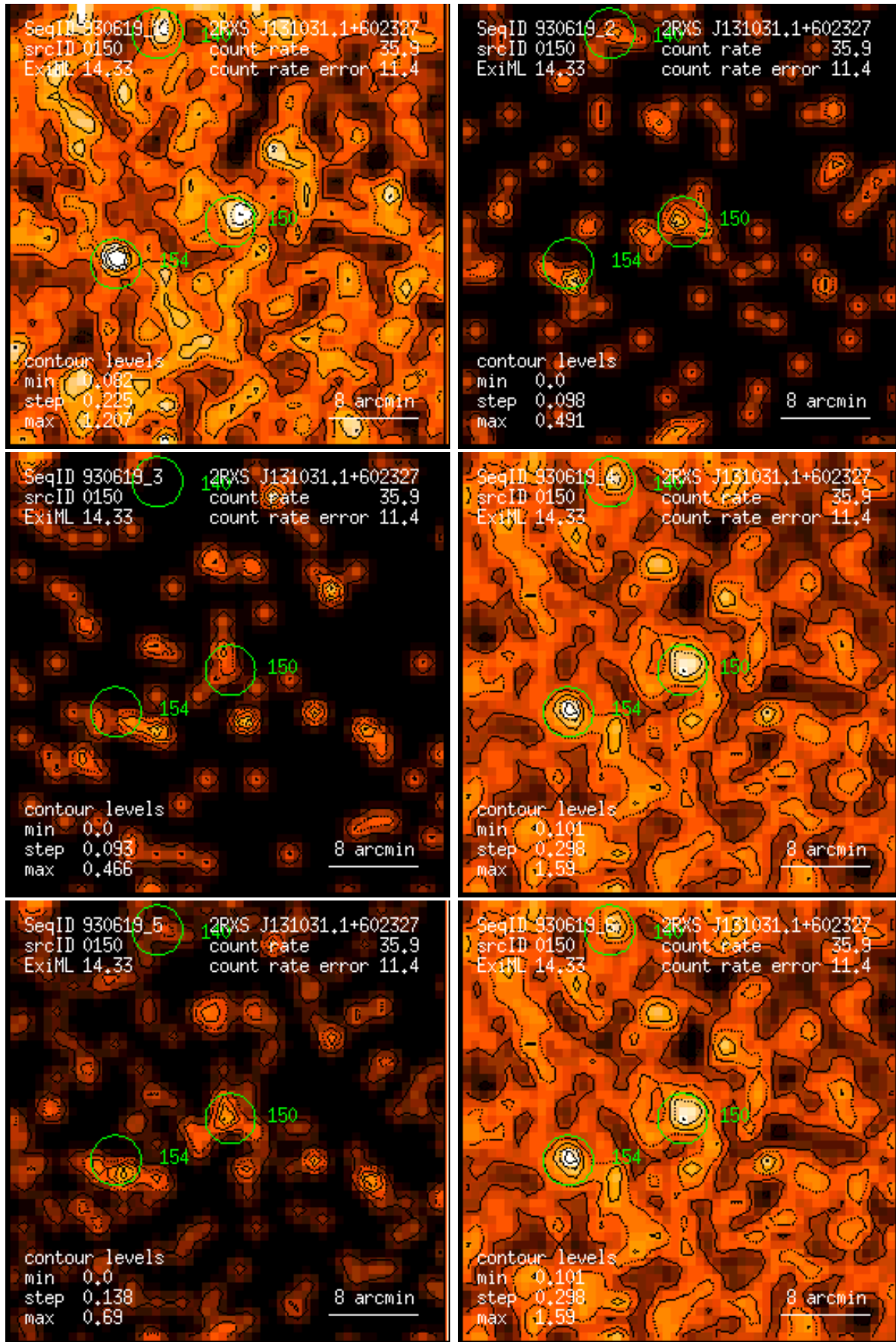
Figure 150: RASS 930619: detection 0150: band rate images, Gaussian filter: (1) PSPC channels 11 – 41, (2) 52 – 90, (3) 91 – 201, (4) 11 – 235, (5) 52 – 201, (6) 11 – 201. Broad band rates in counts/ks. Band rate contour levels in counts/ks/arcmin 2 .
