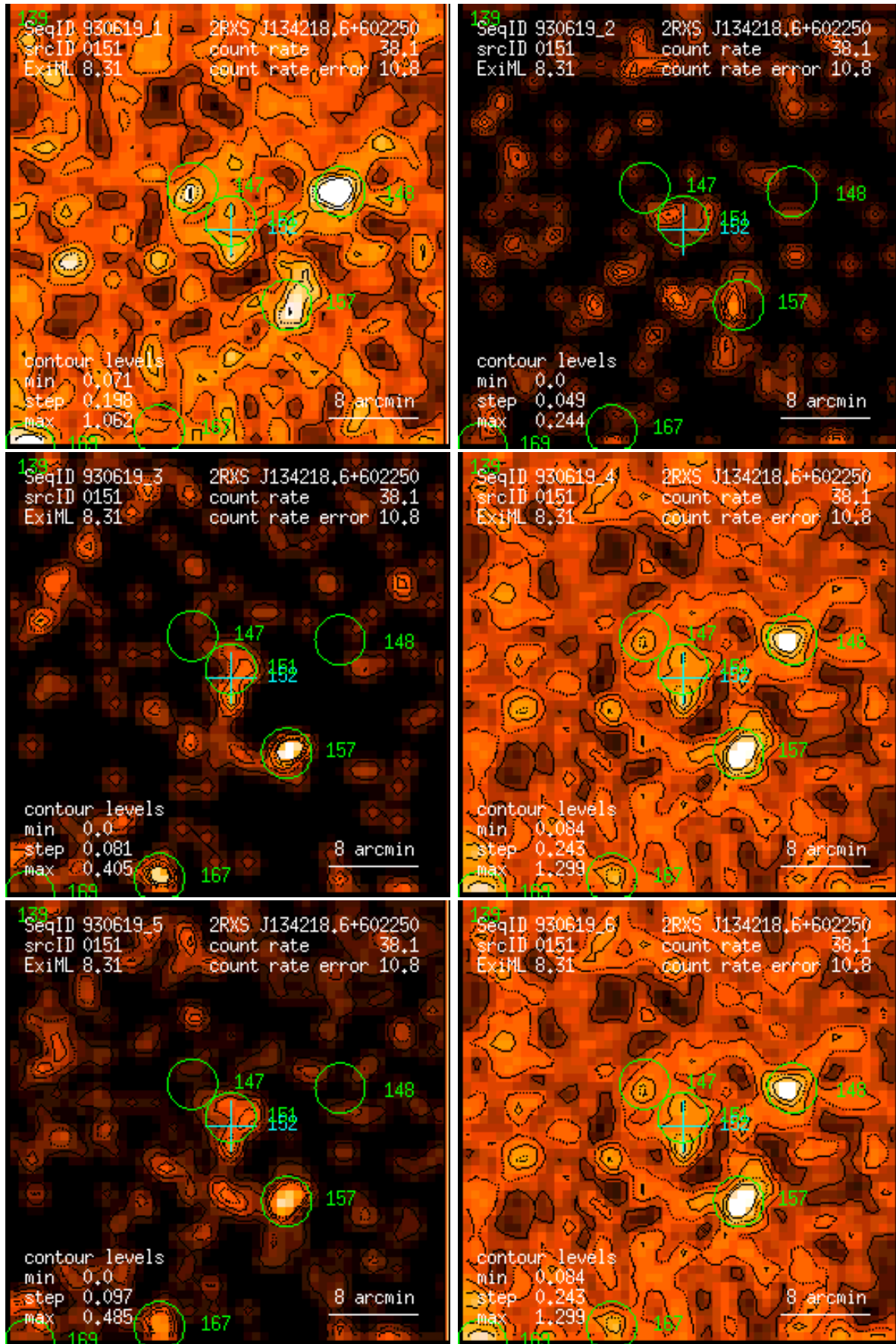
Figure 151: RASS 930619: detection 0151: band rate images, Gaussian filter: (1) PSPC channels 11 – 41, (2) 52 – 90, (3) 91 – 201, (4) 11 – 235, (5) 52 – 201, (6) 11 – 201. Broad band rates in counts/ks. Band rate contour levels in counts/ks/arcmin 2 .
