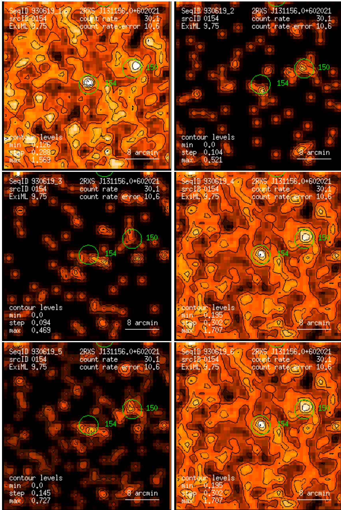
Figure 154: RASS 930619: detection 0154: band rate images, Gaussian filter: (1) PSPC channels 11 – 41, (2) 52 – 90, (3) 91 – 201, (4) 11 – 235, (5) 52 – 201, (6) 11 – 201. Broad band rates in counts/ks. Band rate contour levels in counts/ks/arcmin 2 .
