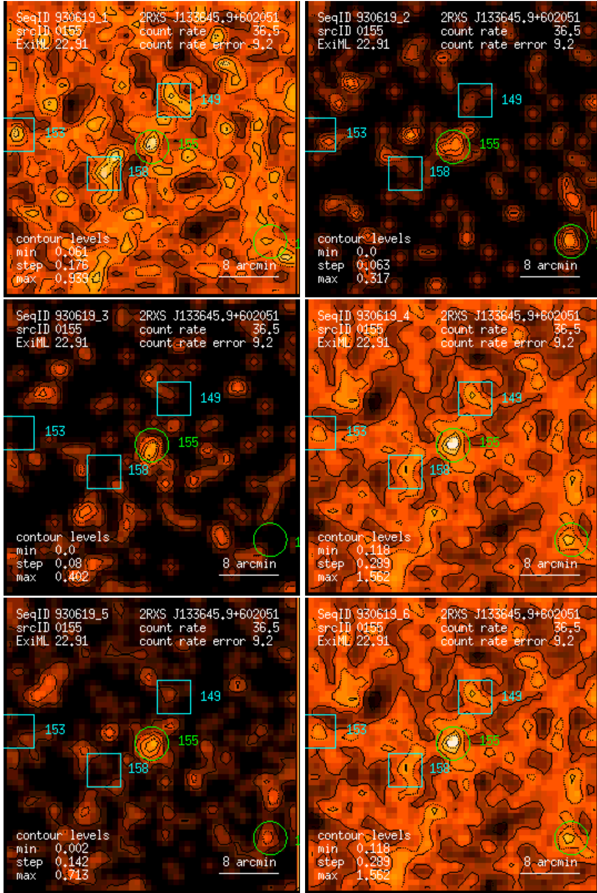
Figure 155: RASS 930619: detection 0155: band rate images, Gaussian filter: (1) PSPC channels 11 – 41, (2) 52 – 90, (3) 91 – 201, (4) 11 – 235, (5) 52 – 201, (6) 11 – 201. Broad band rates in counts/ks. Band rate contour levels in counts/ks/arcmin 2 .
