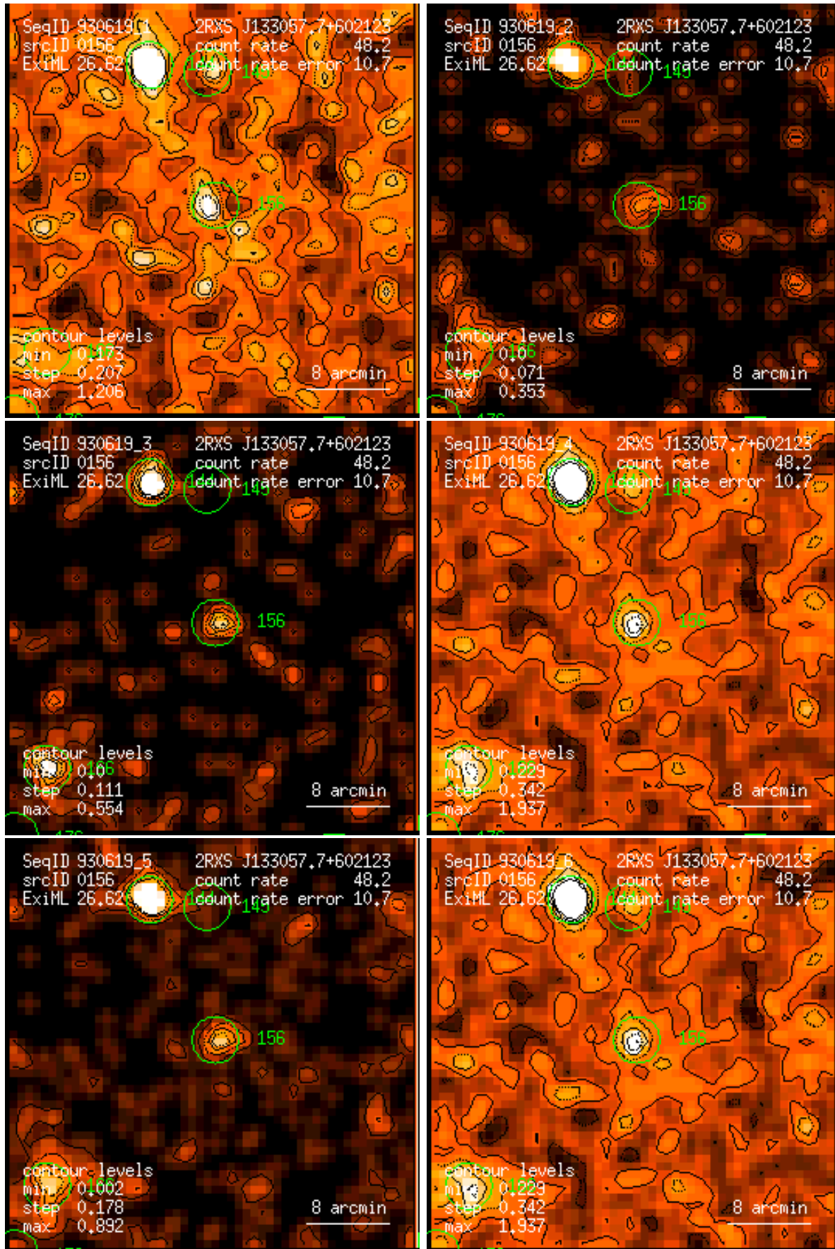
Figure 156: RASS 930619: detection 0156: band rate images, Gaussian filter: (1) PSPC channels 11 – 41, (2) 52 – 90, (3) 91 – 201, (4) 11 – 235, (5) 52 – 201, (6) 11 – 201. Broad band rates in counts/ks. Band rate contour levels in counts/ks/arcmin 2 .
