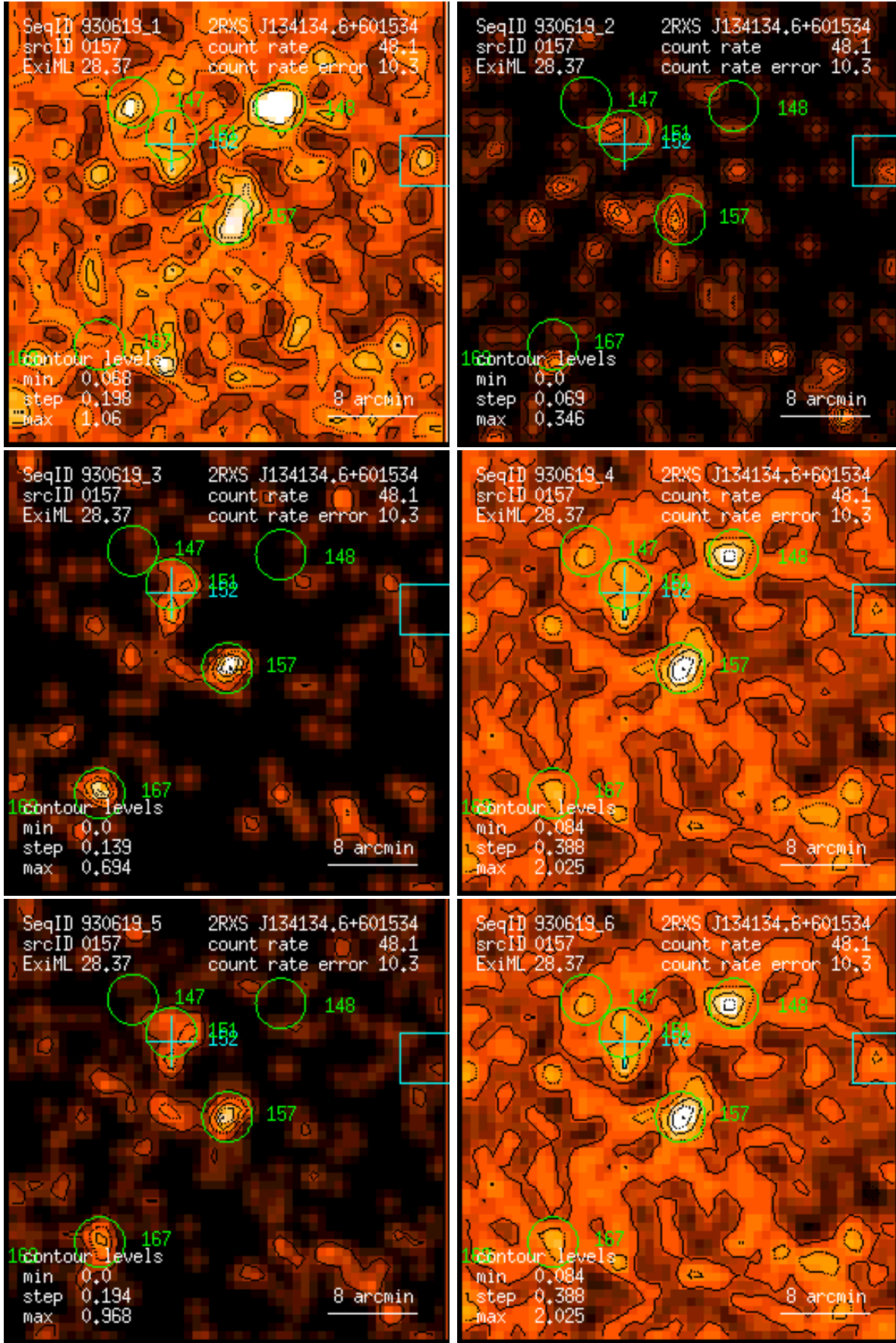
Figure 157: RASS 930619: detection 0157: band rate images, Gaussian filter: (1) PSPC channels 11 – 41, (2) 52 – 90, (3) 91 – 201, (4) 11 – 235, (5) 52 – 201, (6) 11 – 201. Broad band rates in counts/ks. Band rate contour levels in counts/ks/arcmin 2 .
