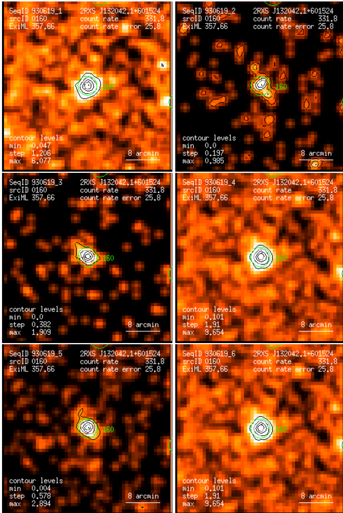
Figure 160: RASS 930619: detection 0160: band rate images, Gaussian filter: (1) PSPC channels 11 – 41, (2) 52 – 90, (3) 91 – 201, (4) 11 – 235, (5) 52 – 201, (6) 11 – 201. Broad band rates in counts/ks. Band rate contour levels in counts/ks/arcmin 2 .
