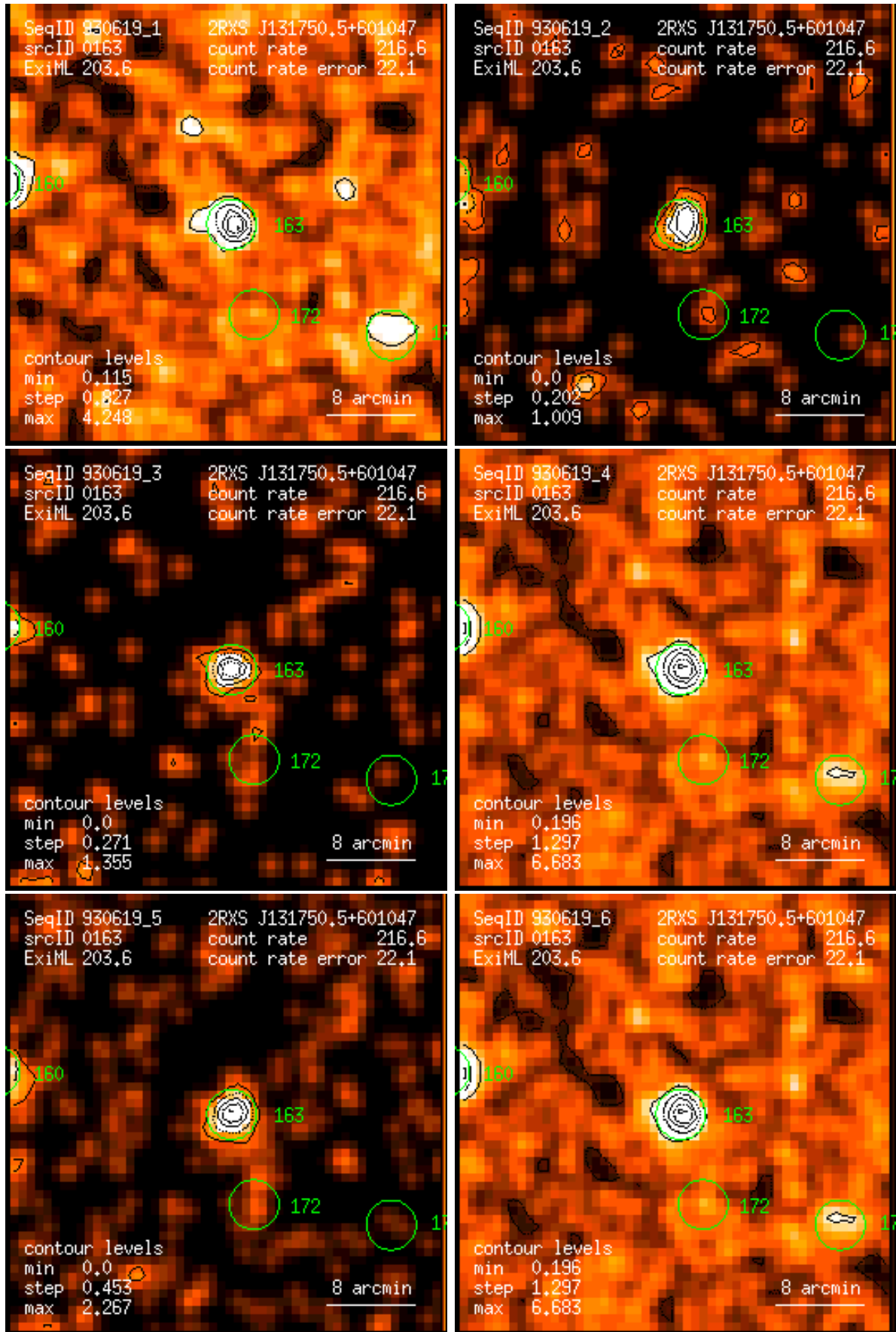
Figure 163: RASS 930619: detection 0163: band rate images, Gaussian filter: (1) PSPC channels 11 – 41, (2) 52 – 90, (3) 91 – 201, (4) 11 – 235, (5) 52 – 201, (6) 11 – 201. Broad band rates in counts/ks. Band rate contour levels in counts/ks/arcmin 2 .
