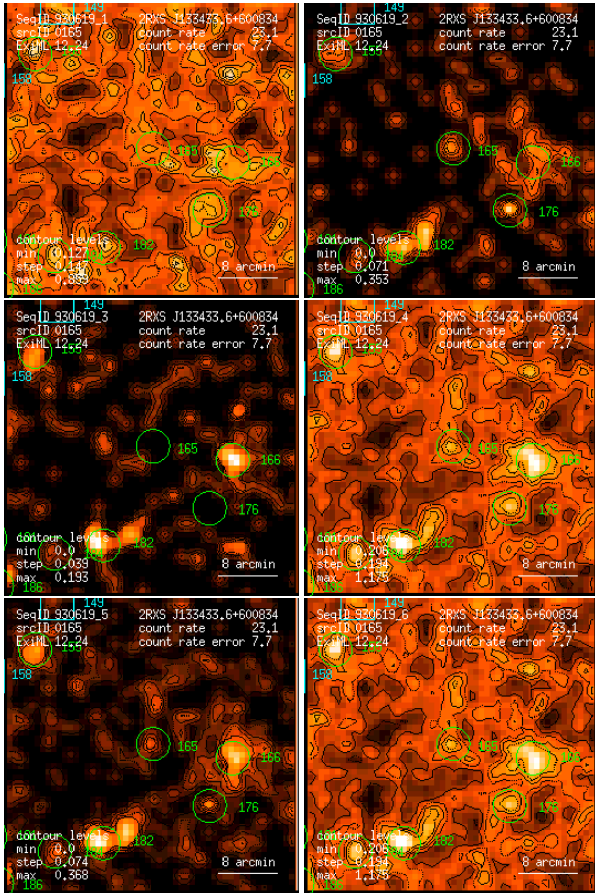
Figure 165: RASS 930619: detection 0165: band rate images, Gaussian filter: (1) PSPC channels 11 – 41, (2) 52 – 90, (3) 91 – 201, (4) 11 – 235, (5) 52 – 201, (6) 11 – 201. Broad band rates in counts/ks. Band rate contour levels in counts/ks/arcmin 2 .
