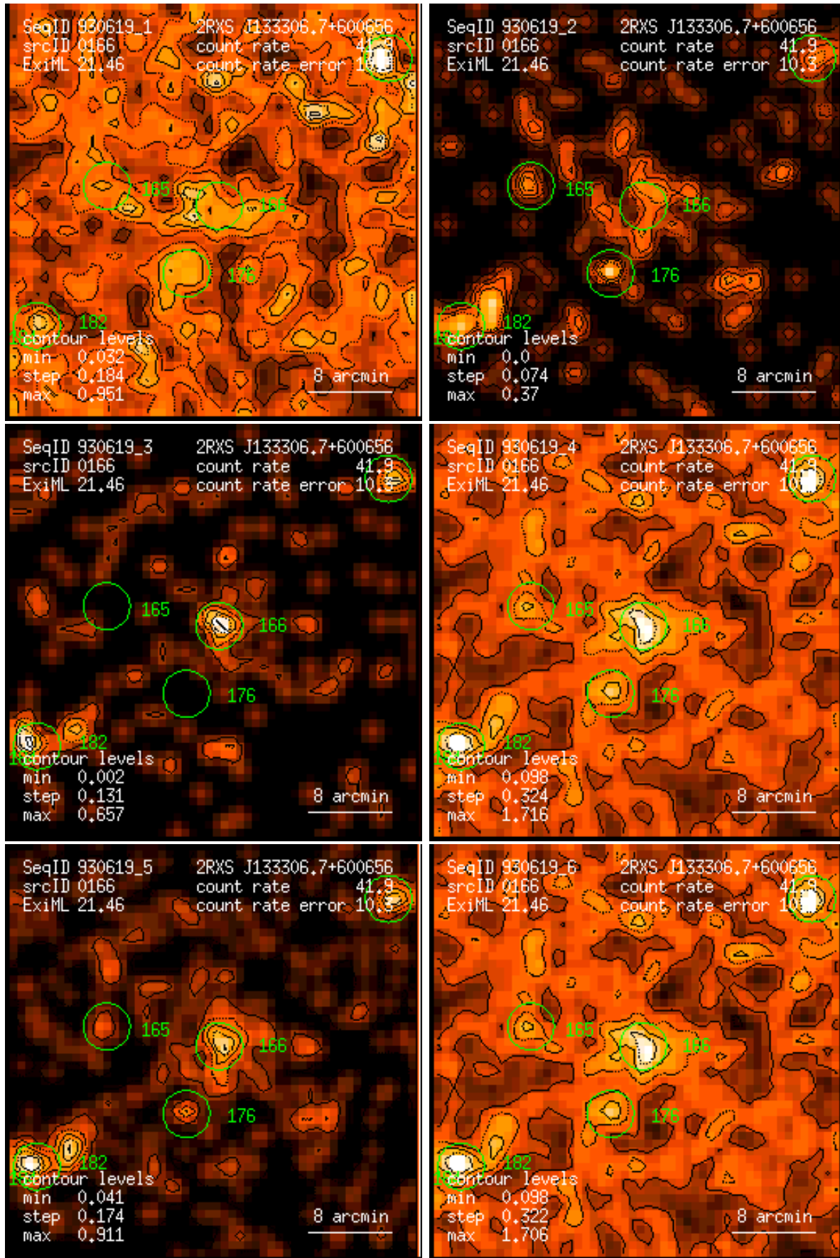
Figure 166: RASS 930619: detection 0166: band rate images, Gaussian filter: (1) PSPC channels 11 – 41, (2) 52 – 90, (3) 91 – 201, (4) 11 – 235, (5) 52 – 201, (6) 11 – 201. Broad band rates in counts/ks. Band rate contour levels in counts/ks/arcmin 2 .
