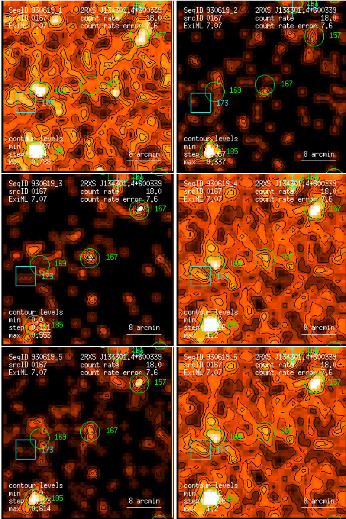
Figure 167: RASS 930619: detection 0167: band rate images, Gaussian filter: (1) PSPC channels 11 – 41, (2) 52 – 90, (3) 91 – 201, (4) 11 – 235, (5) 52 – 201, (6) 11 – 201. Broad band rates in counts/ks. Band rate contour levels in counts/ks/arcmin 2 .
