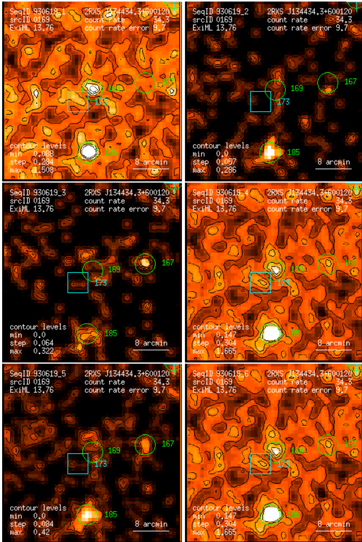
Figure 169: RASS 930619: detection 0169: band rate images, Gaussian filter: (1) PSPC channels 11 – 41, (2) 52 – 90, (3) 91 – 201, (4) 11 – 235, (5) 52 – 201, (6) 11 – 201. Broad band rates in counts/ks. Band rate contour levels in counts/ks/arcmin 2 .
