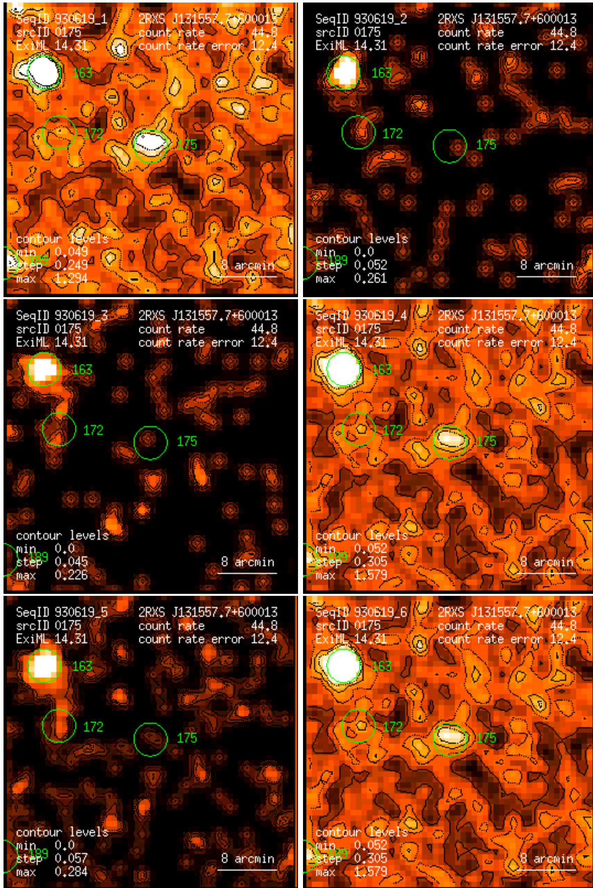
Figure 175: RASS 930619: detection 0175: band rate images, Gaussian filter: (1) PSPC channels 11 – 41, (2) 52 – 90, (3) 91 – 201, (4) 11 – 235, (5) 52 – 201, (6) 11 – 201. Broad band rates in counts/ks. Band rate contour levels in counts/ks/arcmin 2 .
