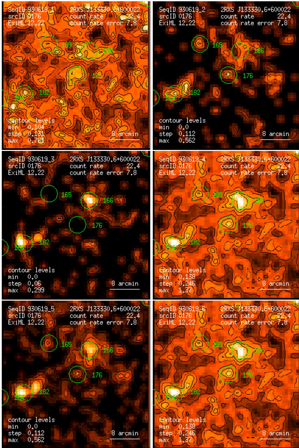
Figure 176: RASS 930619: detection 0176: band rate images, Gaussian filter: (1) PSPC channels 11 – 41, (2) 52 – 90, (3) 91 – 201, (4) 11 – 235, (5) 52 – 201, (6) 11 – 201. Broad band rates in counts/ks. Band rate contour levels in counts/ks/arcmin 2 .
