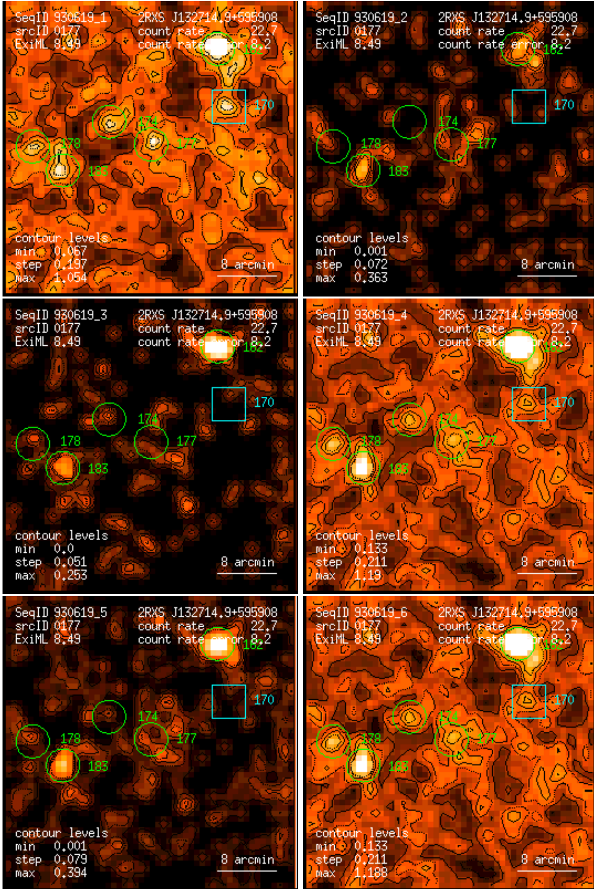
Figure 177: RASS 930619: detection 0177: band rate images, Gaussian filter: (1) PSPC channels 11 – 41, (2) 52 – 90, (3) 91 – 201, (4) 11 – 235, (5) 52 – 201, (6) 11 – 201. Broad band rates in counts/ks. Band rate contour levels in counts/ks/arcmin 2 .
