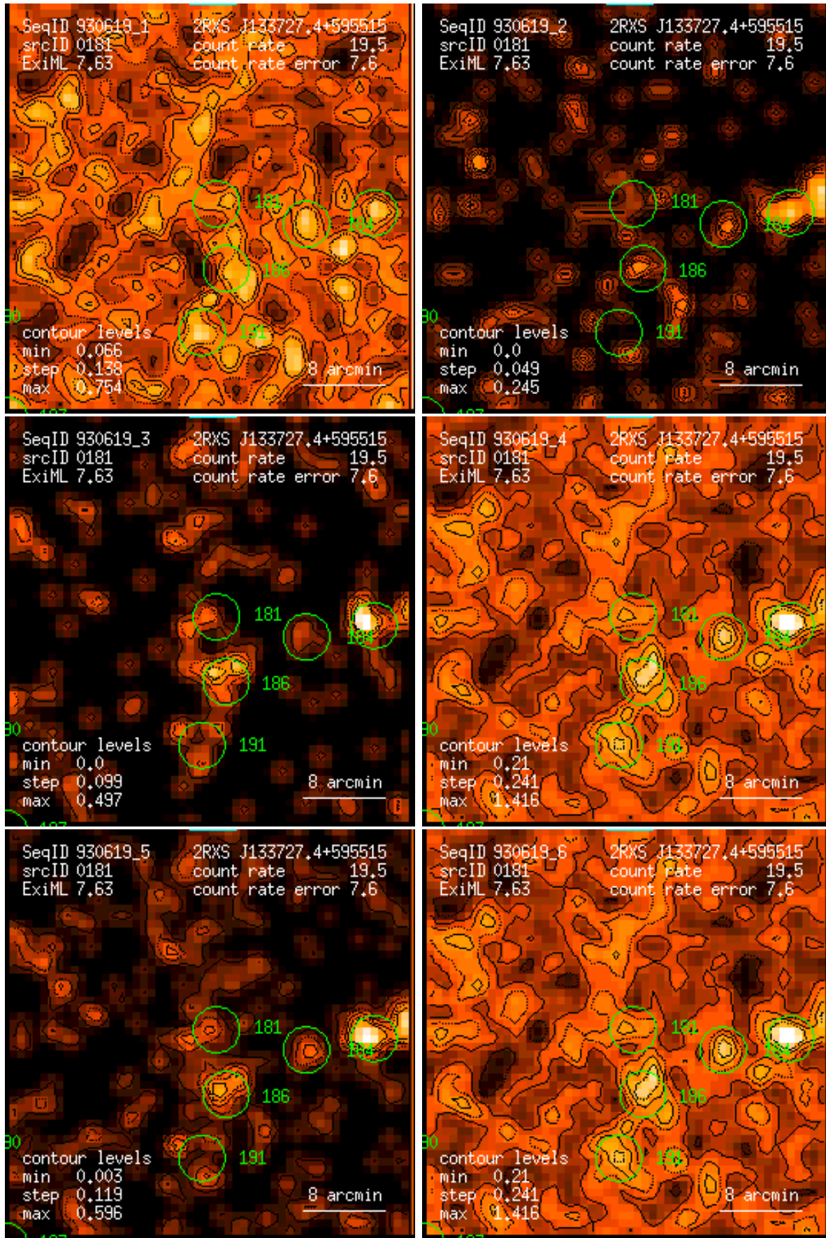
Figure 181: RASS 930619: detection 0181: band rate images, Gaussian filter: (1) PSPC channels 11 – 41, (2) 52 – 90, (3) 91 – 201, (4) 11 – 235, (5) 52 – 201, (6) 11 – 201. Broad band rates in counts/ks. Band rate contour levels in counts/ks/arcmin 2 .
