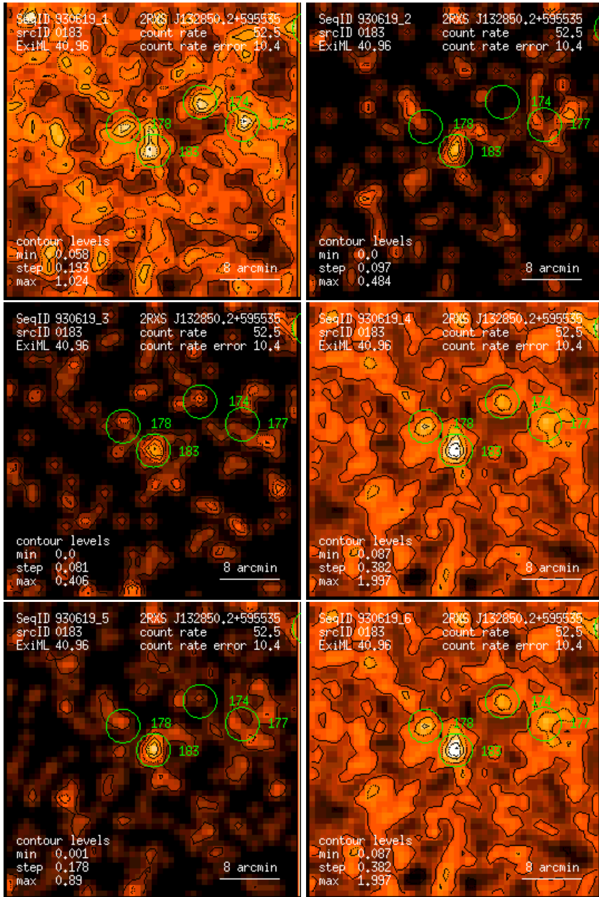
Figure 183: RASS 930619: detection 0183: band rate images, Gaussian filter: (1) PSPC channels 11 – 41, (2) 52 – 90, (3) 91 – 201, (4) 11 – 235, (5) 52 – 201, (6) 11 – 201. Broad band rates in counts/ks. Band rate contour levels in counts/ks/arcmin 2 .
