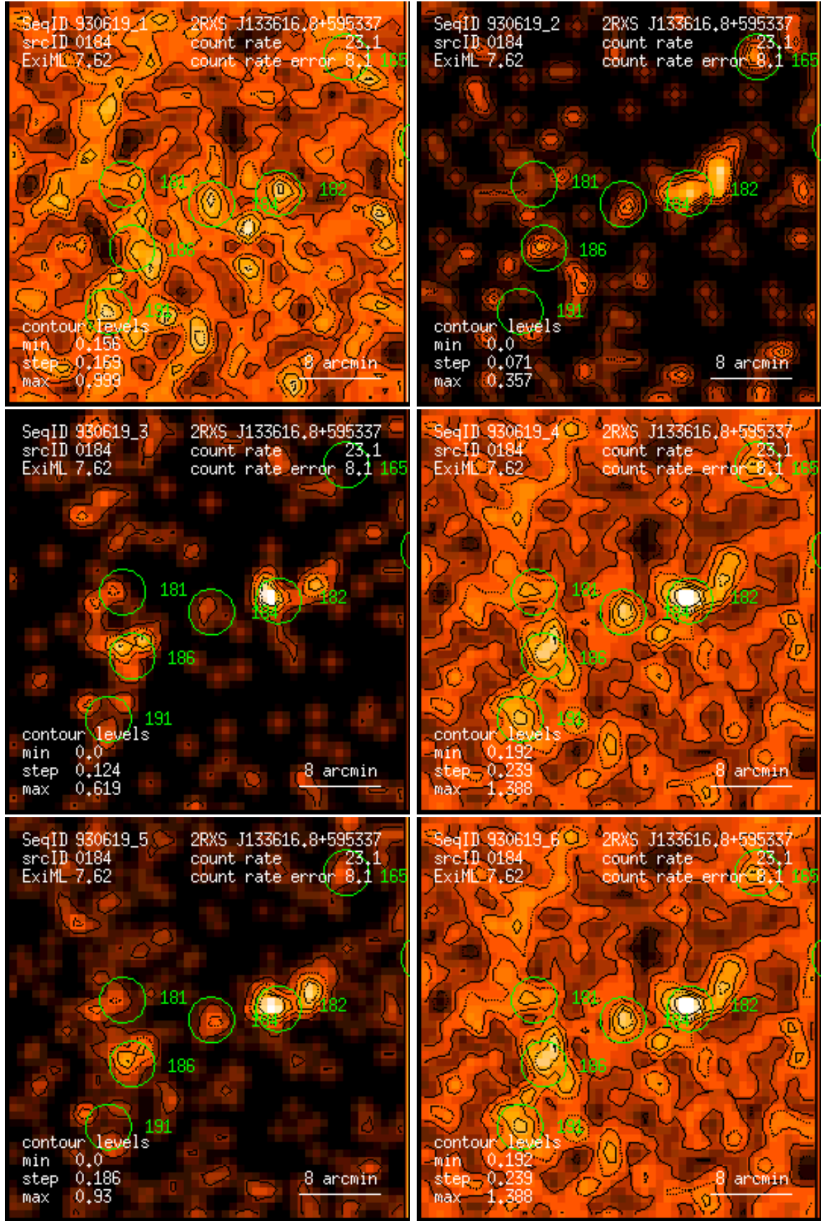
Figure 184: RASS 930619: detection 0184: band rate images, Gaussian filter: (1) PSPC channels 11 – 41, (2) 52 – 90, (3) 91 – 201, (4) 11 – 235, (5) 52 – 201, (6) 11 – 201. Broad band rates in counts/ks. Band rate contour levels in counts/ks/arcmin 2 .
