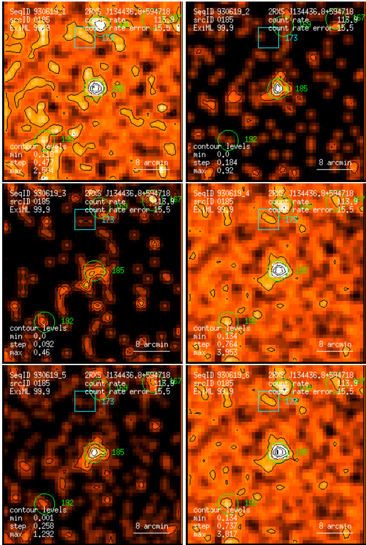
Figure 185: RASS 930619: detection 0185: band rate images, Gaussian filter: (1) PSPC channels 11 – 41, (2) 52 – 90, (3) 91 – 201, (4) 11 – 235, (5) 52 – 201, (6) 11 – 201. Broad band rates in counts/ks. Band rate contour levels in counts/ks/arcmin 2 .
