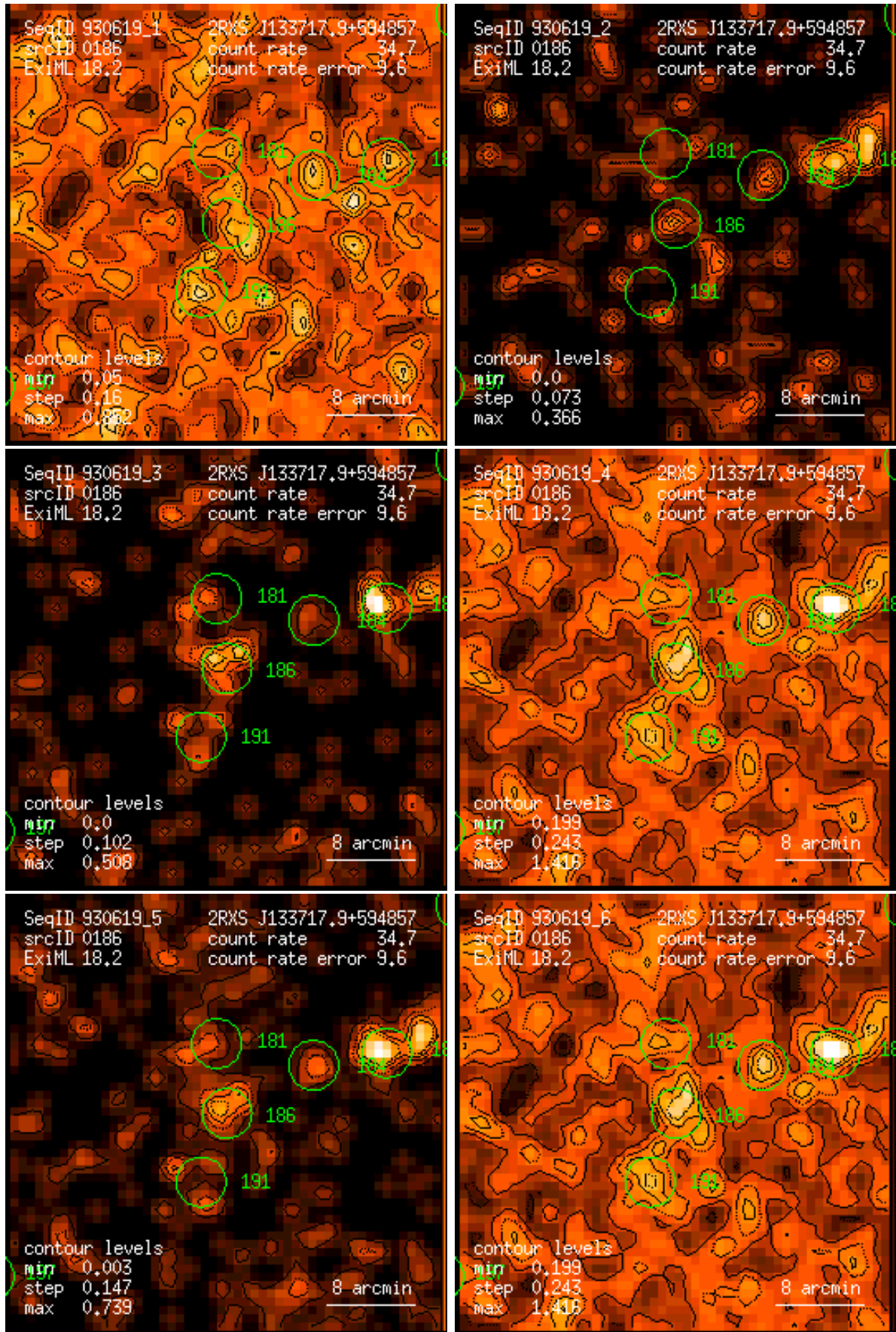
Figure 186: RASS 930619: detection 0186: band rate images, Gaussian filter: (1) PSPC channels 11 – 41, (2) 52 – 90, (3) 91 – 201, (4) 11 – 235, (5) 52 – 201, (6) 11 – 201. Broad band rates in counts/ks. Band rate contour levels in counts/ks/arcmin 2 .
