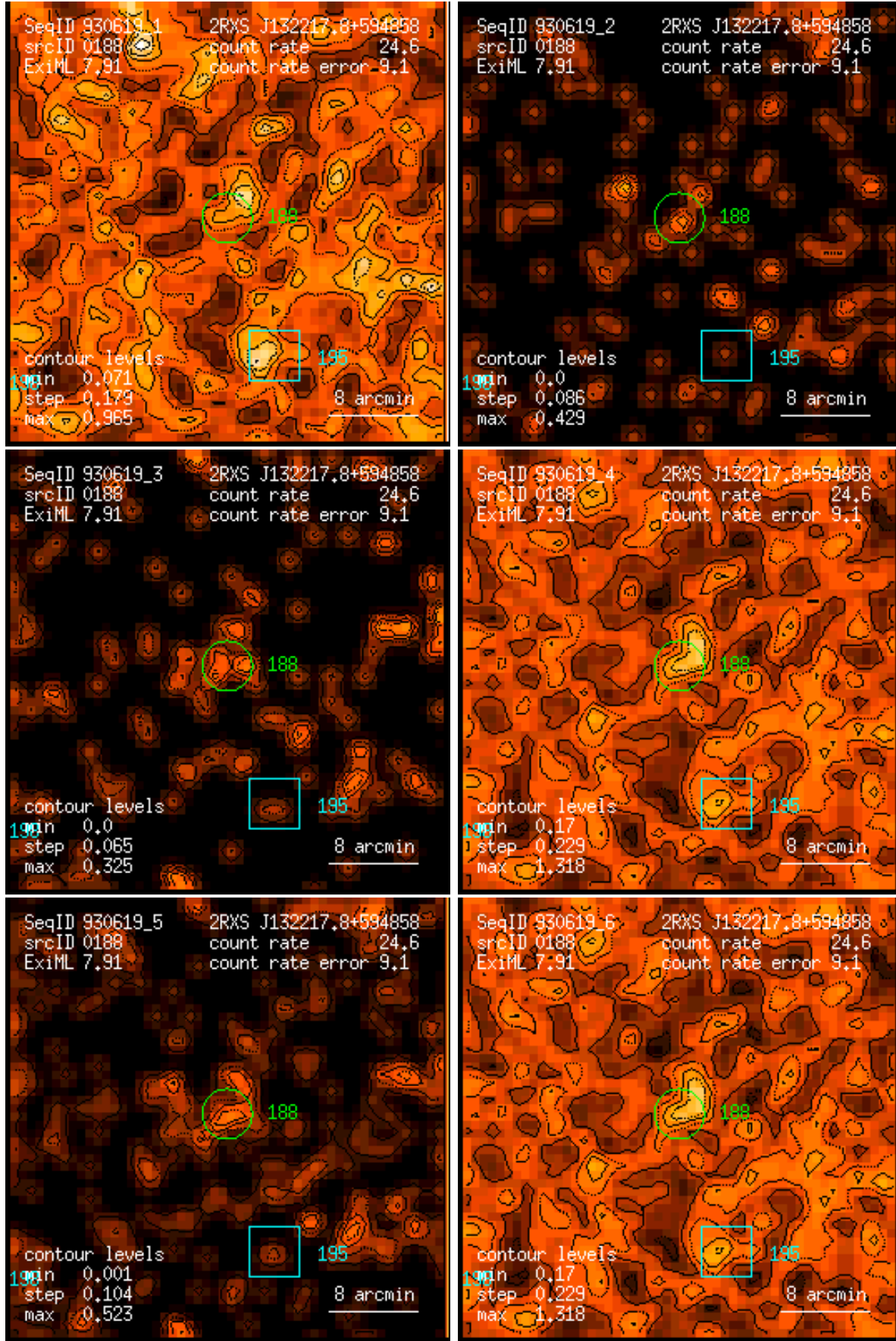
Figure 188: RASS 930619: detection 0188: band rate images, Gaussian filter: (1) PSPC channels 11 – 41, (2) 52 – 90, (3) 91 – 201, (4) 11 – 235, (5) 52 – 201, (6) 11 – 201. Broad band rates in counts/ks. Band rate contour levels in counts/ks/arcmin 2 .
