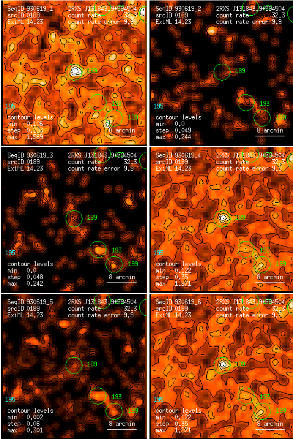
Figure 189: RASS 930619: detection 0189: band rate images, Gaussian filter: (1) PSPC channels 11 – 41, (2) 52 – 90, (3) 91 – 201, (4) 11 – 235, (5) 52 – 201, (6) 11 – 201. Broad band rates in counts/ks. Band rate contour levels in counts/ks/arcmin 2 .
