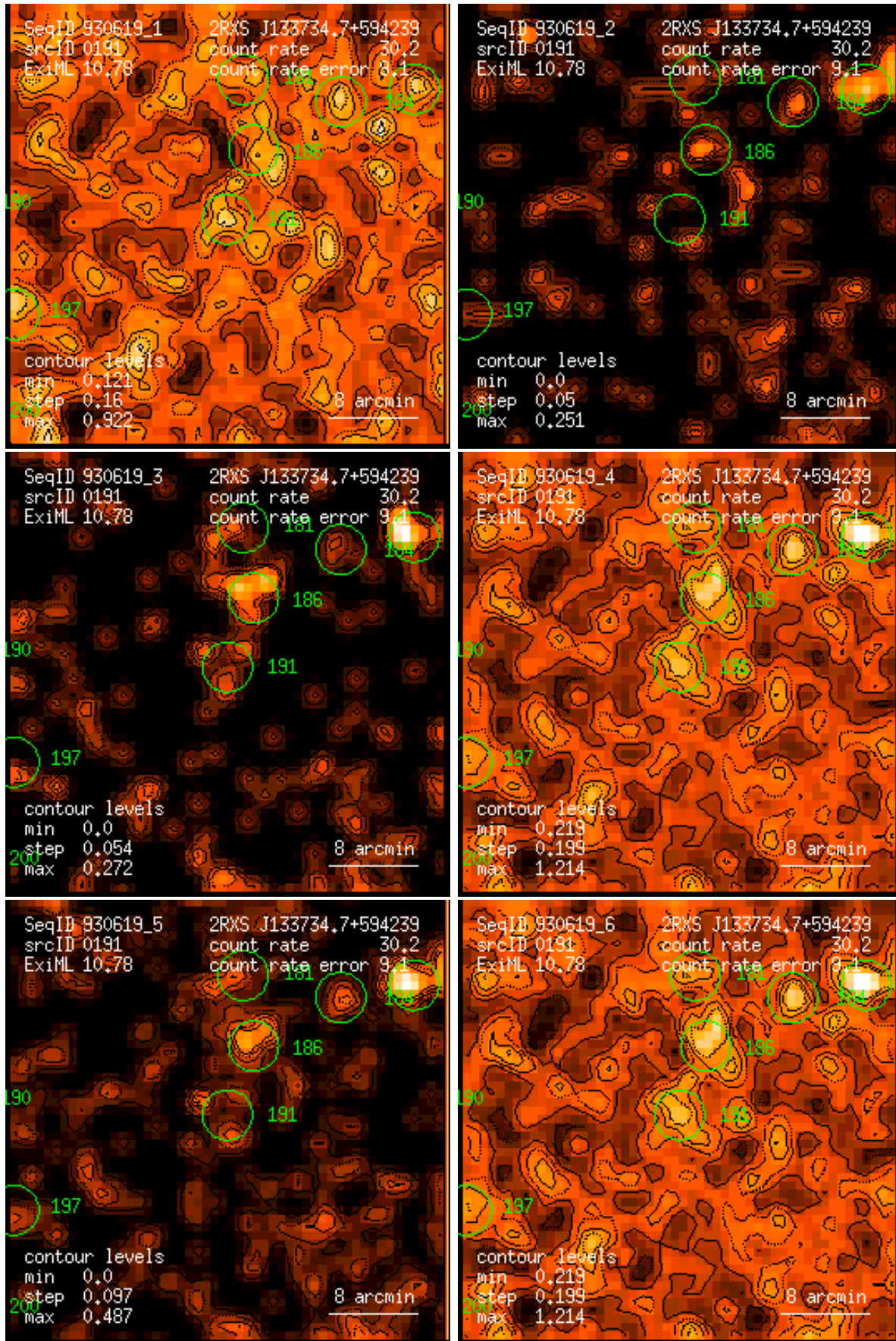
Figure 191: RASS 930619: detection 0191: band rate images, Gaussian filter: (1) PSPC channels 11 – 41, (2) 52 – 90, (3) 91 – 201, (4) 11 – 235, (5) 52 – 201, (6) 11 – 201. Broad band rates in counts/ks. Band rate contour levels in counts/ks/arcmin 2 .
