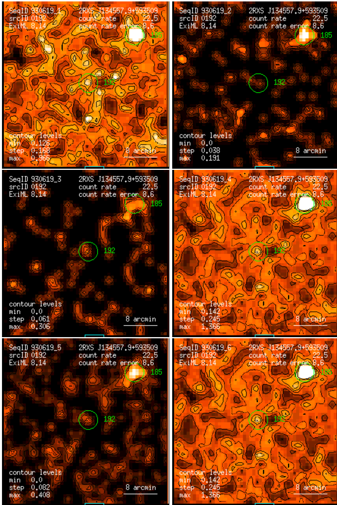
Figure 192: RASS 930619: detection 0192: band rate images, Gaussian filter: (1) PSPC channels 11 – 41, (2) 52 – 90, (3) 91 – 201, (4) 11 – 235, (5) 52 – 201, (6) 11 – 201. Broad band rates in counts/ks. Band rate contour levels in counts/ks/arcmin 2 .
