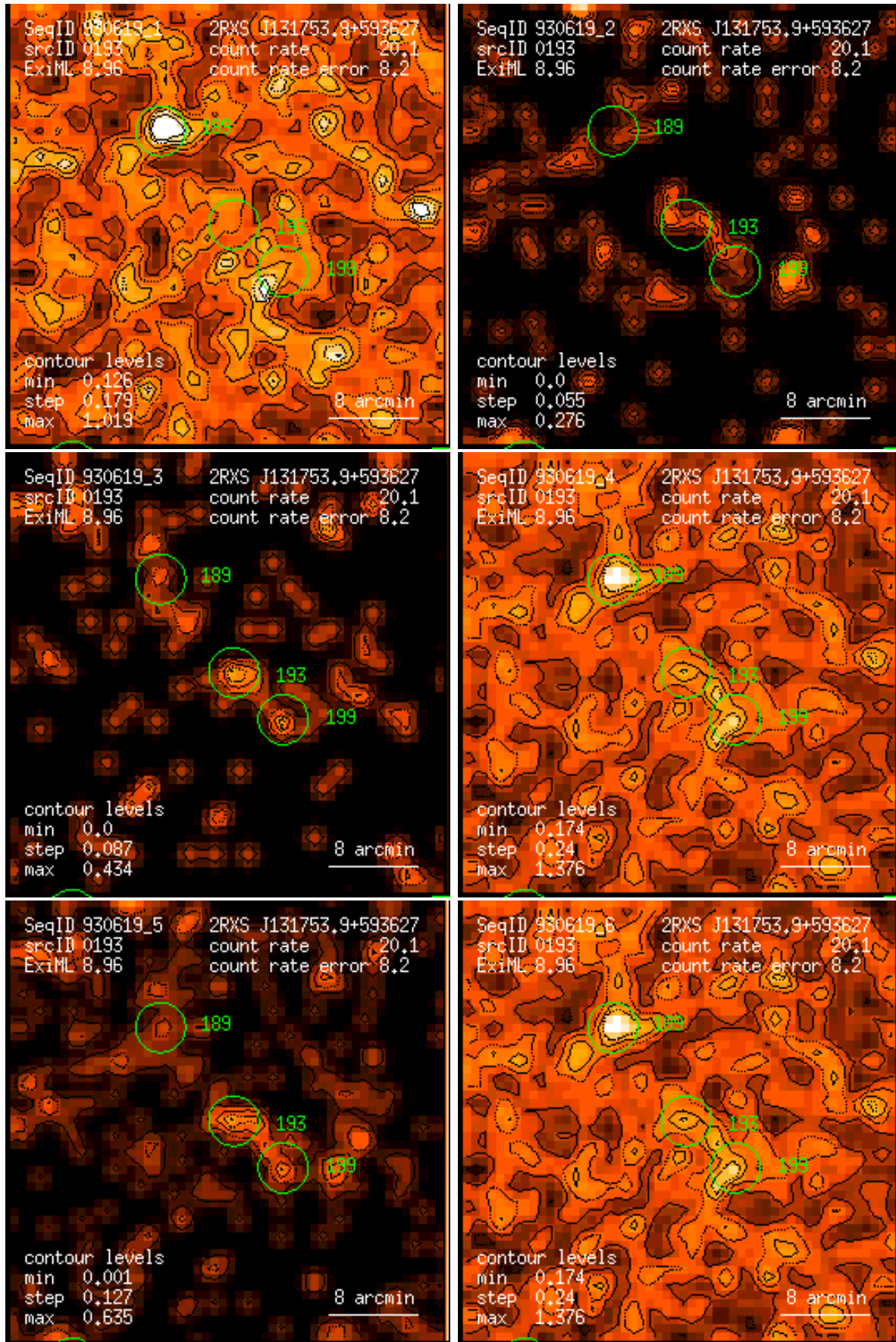
Figure 193: RASS 930619: detection 0193: band rate images, Gaussian filter: (1) PSPC channels 11 – 41, (2) 52 – 90, (3) 91 – 201, (4) 11 – 235, (5) 52 – 201, (6) 11 – 201. Broad band rates in counts/ks. Band rate contour levels in counts/ks/arcmin 2 .
