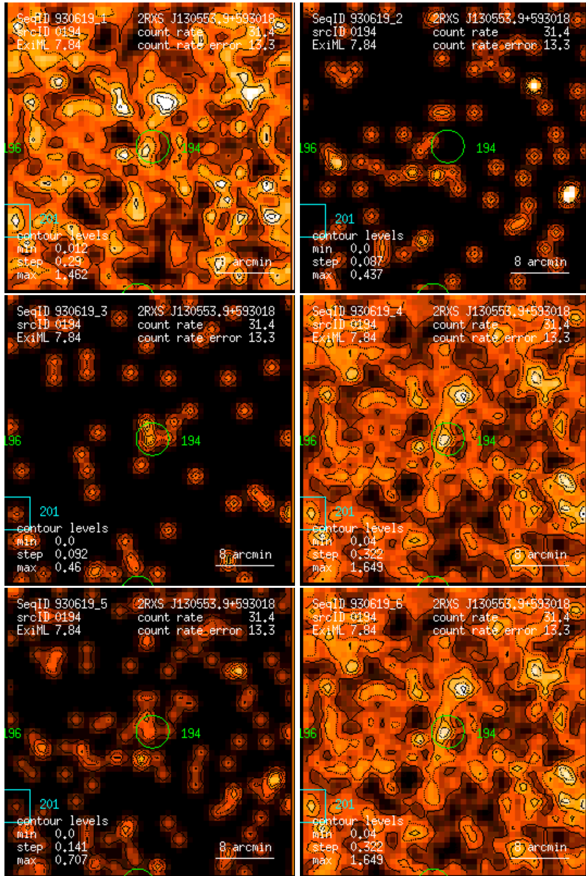
Figure 194: RASS 930619: detection 0194: band rate images, Gaussian filter: (1) PSPC channels 11 – 41, (2) 52 – 90, (3) 91 – 201, (4) 11 – 235, (5) 52 – 201, (6) 11 – 201. Broad band rates in counts/ks. Band rate contour levels in counts/ks/arcmin 2 .
