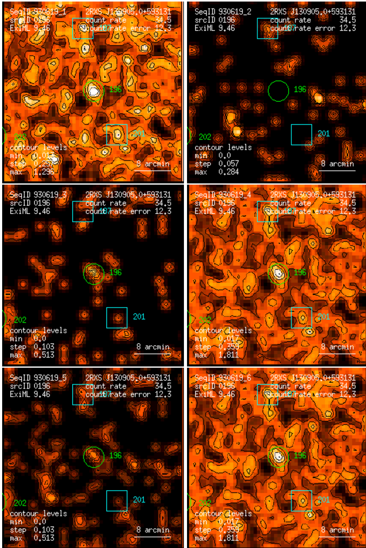
Figure 196: RASS 930619: detection 0196: band rate images, Gaussian filter: (1) PSPC channels 11 – 41, (2) 52 – 90, (3) 91 – 201, (4) 11 – 235, (5) 52 – 201, (6) 11 – 201. Broad band rates in counts/ks. Band rate contour levels in counts/ks/arcmin 2 .
