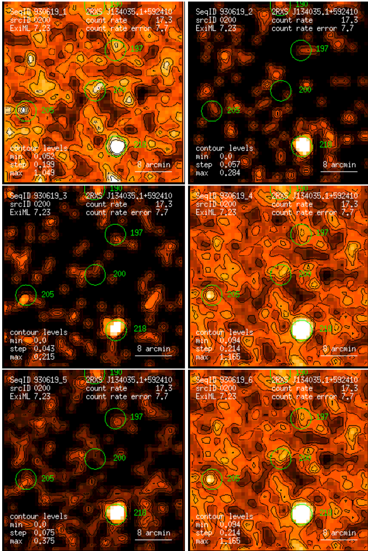
Figure 200: RASS 930619: detection 0200: band rate images, Gaussian filter: (1) PSPC channels 11 – 41, (2) 52 – 90, (3) 91 – 201, (4) 11 – 235, (5) 52 – 201, (6) 11 – 201. Broad band rates in counts/ks. Band rate contour levels in counts/ks/arcmin 2 .
