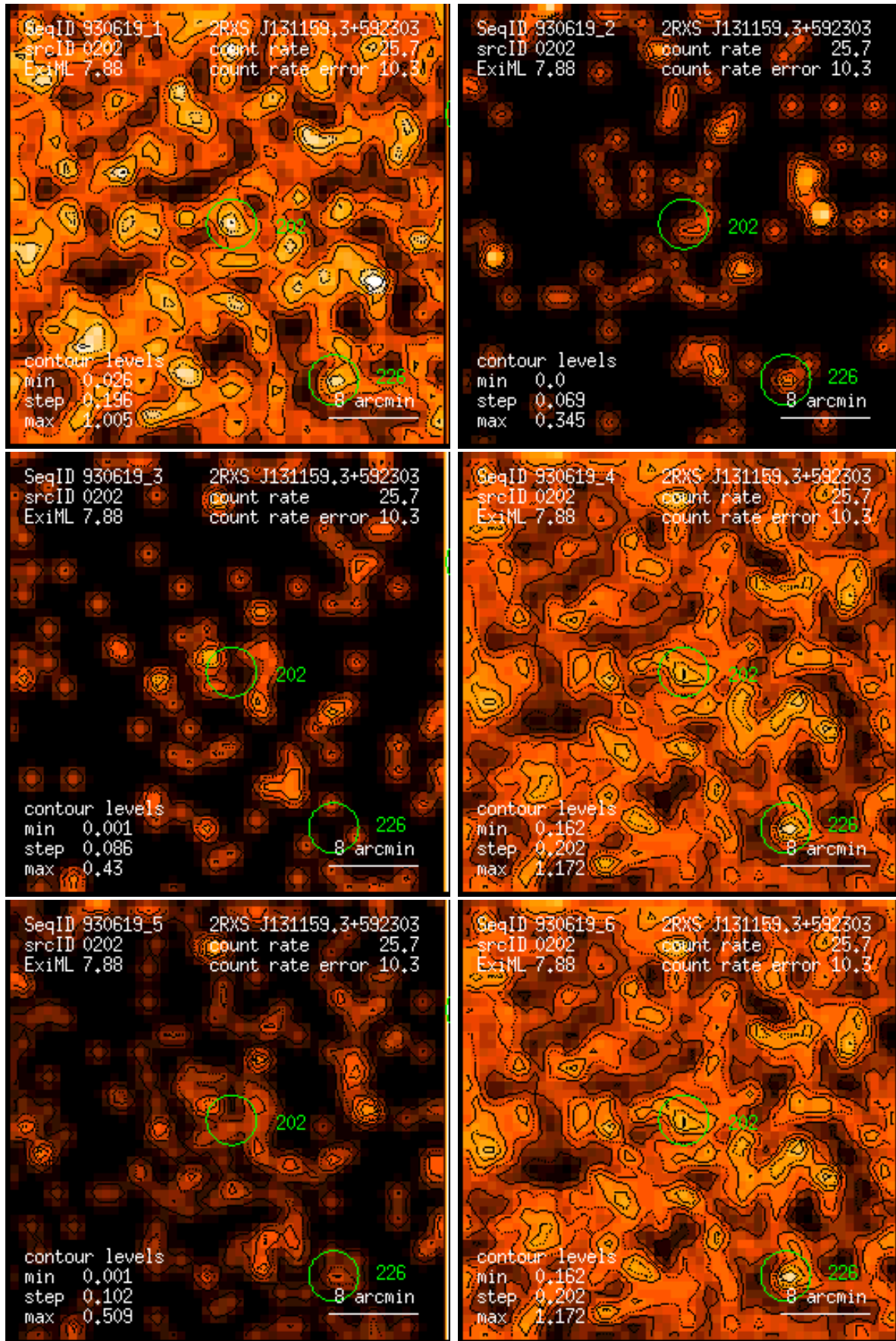
Figure 202: RASS 930619: detection 0202: band rate images, Gaussian filter: (1) PSPC channels 11 – 41, (2) 52 – 90, (3) 91 – 201, (4) 11 – 235, (5) 52 – 201, (6) 11 – 201. Broad band rates in counts/ks. Band rate contour levels in counts/ks/arcmin 2 .
